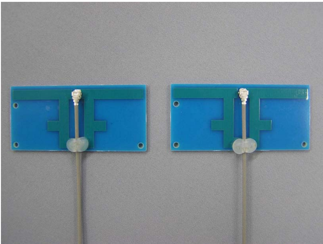
Rear View of LFANT 103
