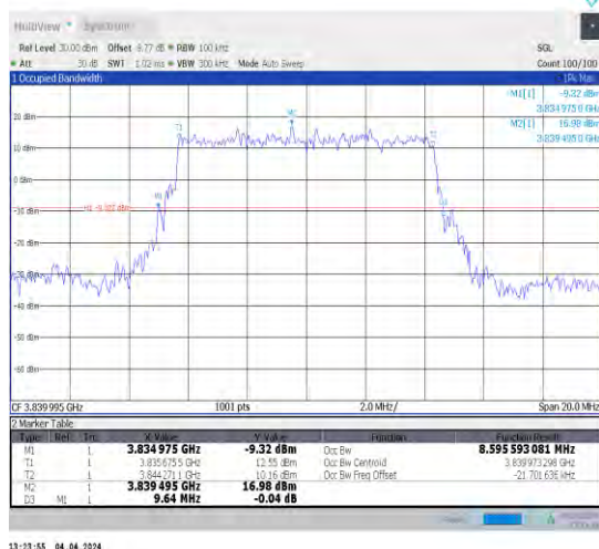
1-N77-3700-3980-30-10-M-2-DFT-PI2BPSK-Outer_Full-24@0-Ant1-8.596-9.640-≤10-PASS
