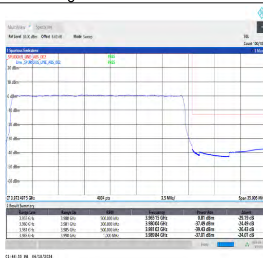
1-N77-3700-3980-30-25-H-3-DFT-PI2BPSK-Outer_Full-64@0-Ant1-1--PASS-see graph
