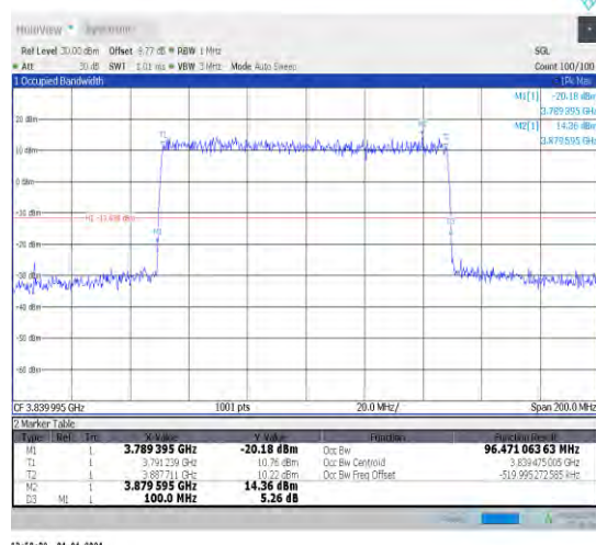
1-N77-3700-3980-30-100-M-4-DFT-64QAM-Outer_Full-270@0-Ant1-96.471-100.000-≤100-PASS
