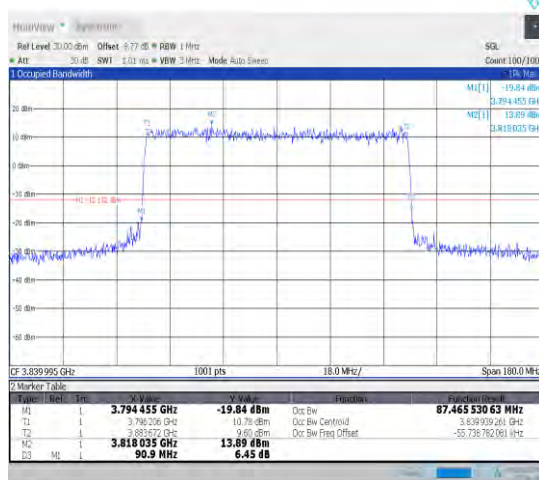
1-N77-3700-3980-30-90-M-8-CP-64QAM-Out_Full- 245@0-Ant1-87.466-90.900≤90-PASS
