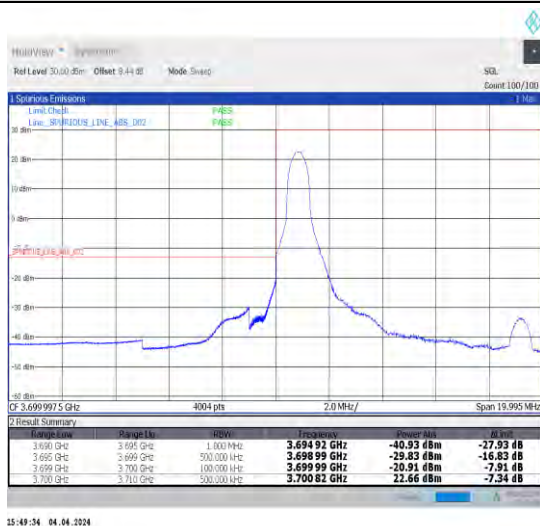
1-N77-3700-3980-30-10-L-4-CP-QPSK-Edge_1RB_Lef t-1@0-Ant1-1--PASS-see graph
