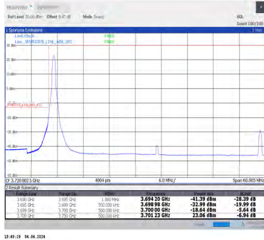
1-N77-3700-3980-30-50-L-1-DFT-PI2BPSK-Edge_1RB _Left-1@0-Ant1-1--PASS-see graph
