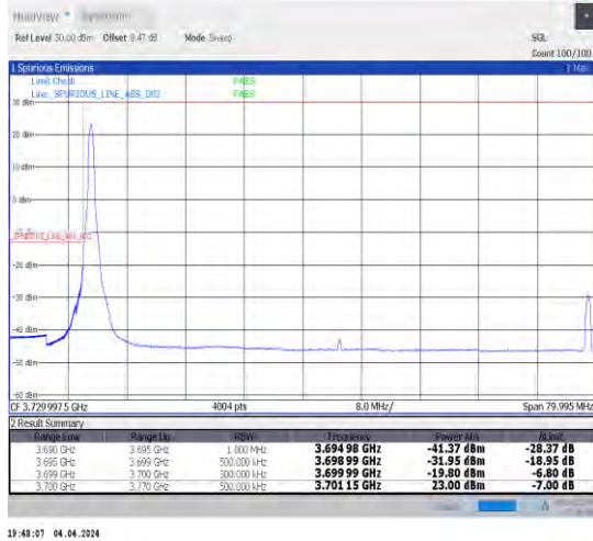
1-N77-3700-3980-30-70-L-1-DFT-PI2BPSK-Edge_1RB _Left-1@0-Ant1-1--PASS-see graph
