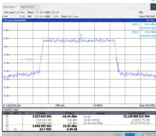
1-N77-3700-3980-30-25-M-9-CP-256QAM-Outer_Ful I-65@0-Ant1-23.151-24.700-≤25-PASS
