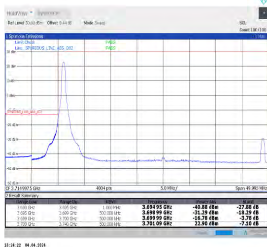
1-N77-3700-3980-30-40-L-4-CP-QPSK-Edge_1RB_Lef t-1@0-Ant1-1--PASS-see graph
