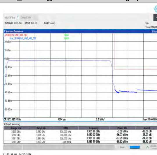
1-N77-3700-3980-30-25-H-6-CP-QPSK-Outer_Full-65@0-Ant1-1--PASS-see graph
