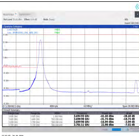
1-N77-3700-3980-30-30-L-1-DFT-PI2BPSK-Edge_1RB _Left-1@0-Ant1-1--PASS-see graph
