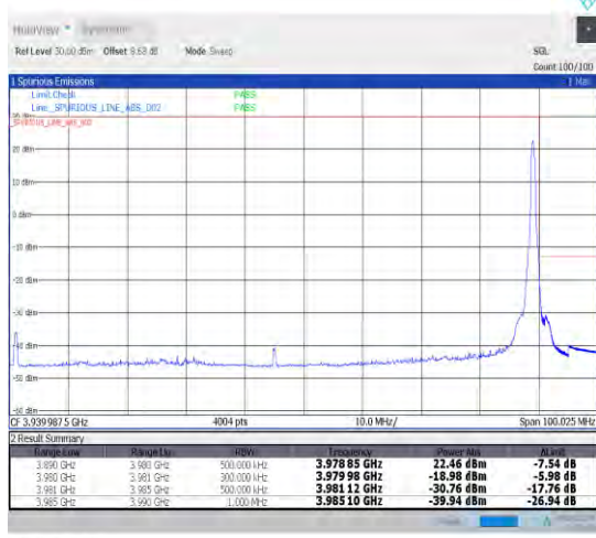
1-N77-3700-3980-30-90-H-5-CP-QPSK-Edge_1RB_Ri ght-1@244-Ant1-1--PASS-see graph
