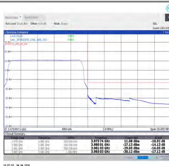
1-N77-3700-3980-30-10-H-6-CP-QPSK-Outer_Full-24@0-Ant1-1--PASS-see graph
