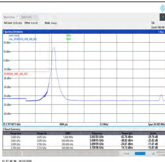
1-N77-3700-3980-30-25-L-1-DFT-PI2BPSK-Edge_1RB_Left-1@0-Ant1-1--PASS-see graph
