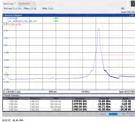
1-N77-3700-3980-30-30-H-2-DFT-PI2BPSK-Edge_1R B_Right-1@77-Ant1-1--PASS-see graph
