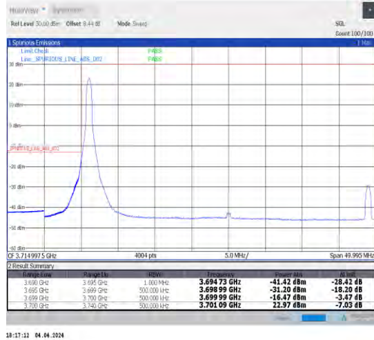
1-N77-3700-3980-30-40-L-1-DFT-PI2BPSK-Edge_1RB _Left-1@0-Ant1-1--PASS-see graph
