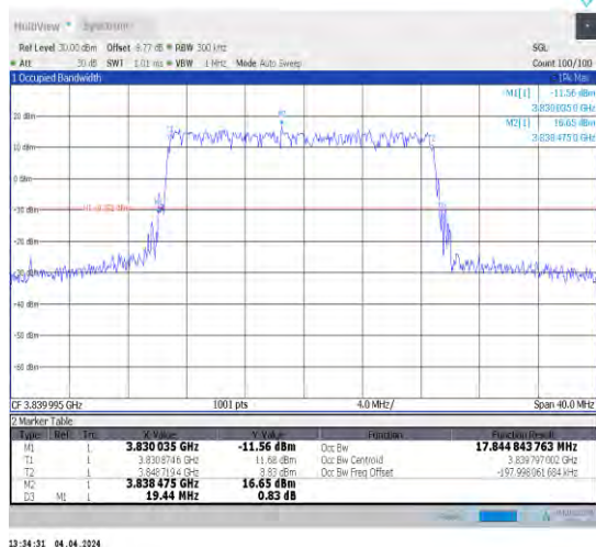
1-N77-3700-3980-30-20-M-3-DFT-16QAM-Outer_Full-50@0-Ant1-17.845-19.440-≤20-PASS
