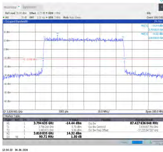
1-N77-3700-3980-30-90-M-6-CP-QPSK-Out_Full-2 45@0-Ant1-87.428-90.720≤90-PASS
