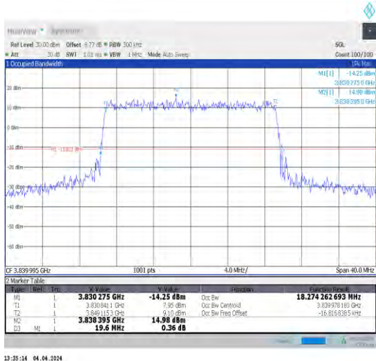
1-N77-3700-3980-30-20-M-8-CP-64QAM-Outer_Full-51@0-Ant1-18.274-19.600-≤20-PASS
