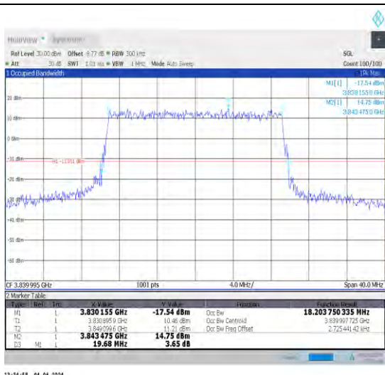
1-N77-3700-3980-30-20-M-6-CP-QPSK-Outer_Full-5 1@0-Ant1-18.204-19.680-≤20-PASS
