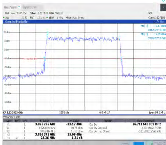
1-N77-3700-3980-30-30-M-1-DFT-QPSK-Outer_Full-75@0-Ant1-26.712-28.260-≤30-PASS
