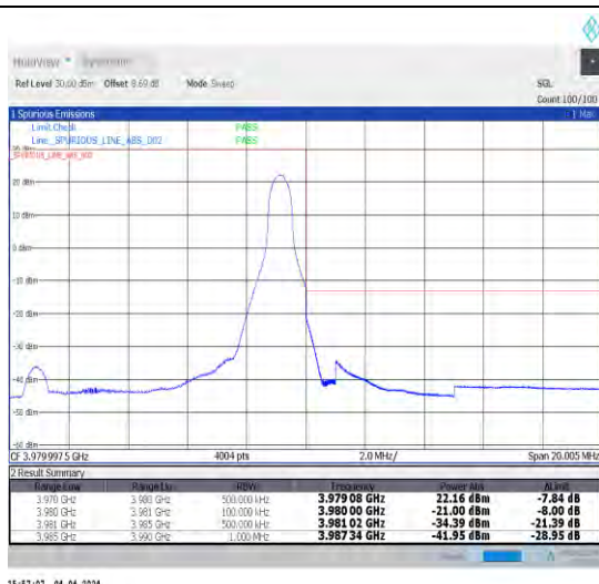
1-N77-3700-3980-30-10-H-2-DFT-PI2BPSK-Edge_1R_B_Right-1@23-Ant1-1--PASS-see graph
