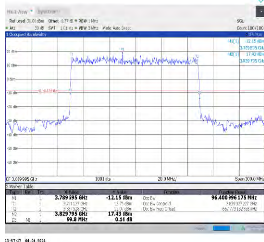
1-N77-3700-3980-30-100-M-2-DFT-PI2BPSK-Outer_Full-270@0-Ant1-96.401-99.800-≤100-PASS
