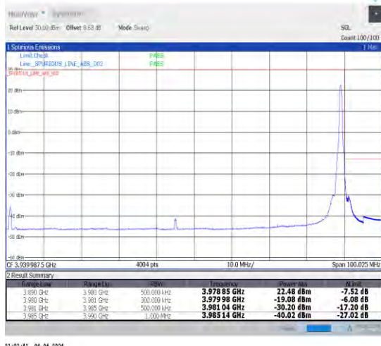
1-N77-3700-3980-30-90-H-2-DFT-PI2BPSK-Edge_1R B_Right-1@244-Ant1-1--PASS-see graph
