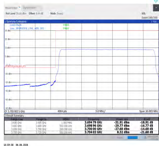
1-N77-3700-3980-30-20-L-6-CP-QPSK-Outer_Full -51@0-Ant1-1--PASS-see graph
