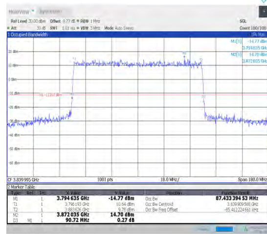
1-N77-3700-3980-30-90-M-7-CP-16QAM-Out_Full -245@0-Ant1-87.433-90.720≤90-PASS
