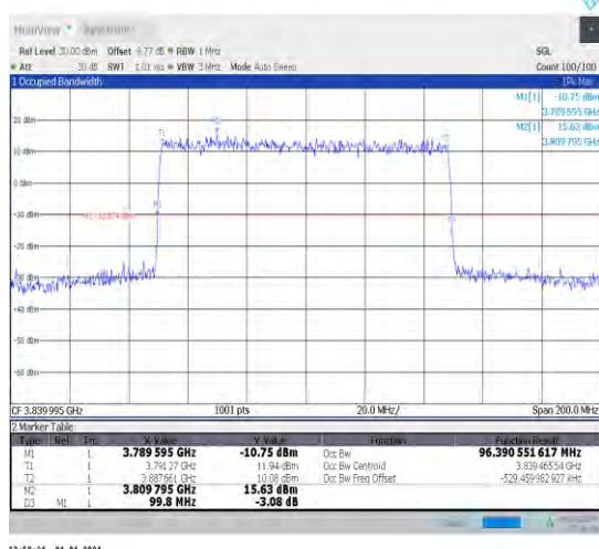
1-N77-3700-3980-30-100-M-3-DFT-16QAM-Outer_Full-270@0-Ant1-96.391-99.800-≤100-PASS
