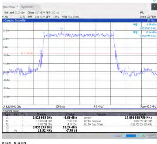
1-N77-3700-3980-30-20-M-2-DFT-PI2BPSK-Outer_Full-50@0-Ant1-17.897-19.520-≤20-PASS
