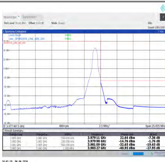
1-N77-3700-3980-30-15-H-5-CP-QPSK-Edge_1RB_Right-1@37-Ant1-1--PASS-see graph
