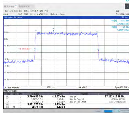
1-N77-3700-3980-30-90-M-9-CP-256QAM-Out_Fu ll-245@0-Ant1-87.282-90.720≤90-PASS
