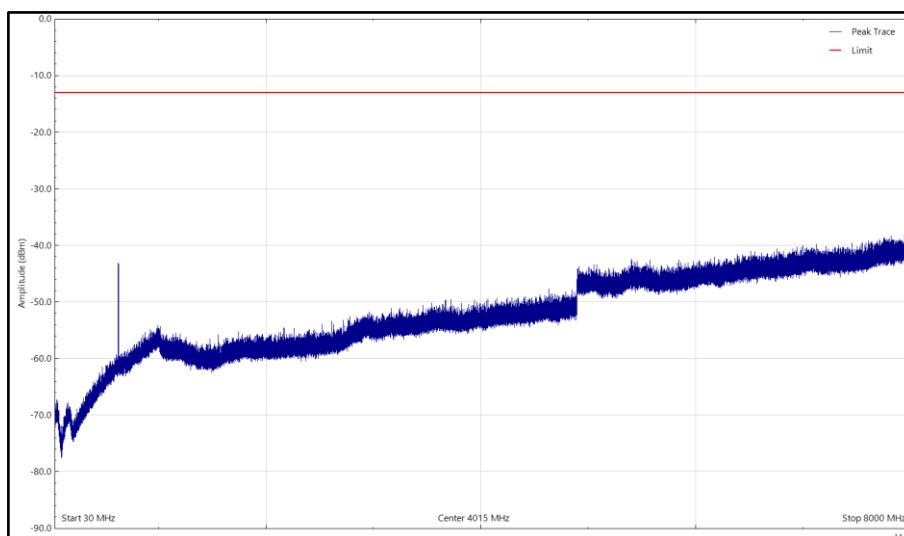
Bot - NR&NB-IoT - B71, 622MHz, 30 MHz to 8 GHz, Vertical (Peak)
