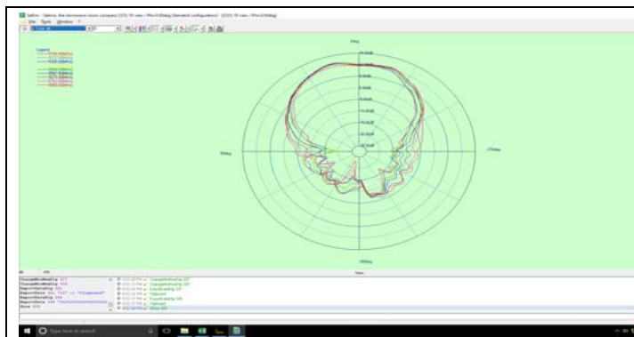
2D radiation direction diagram of horizontally polarized Port (Plane H)
