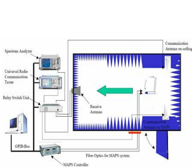
(Testing by 3D anechoic chamber)
