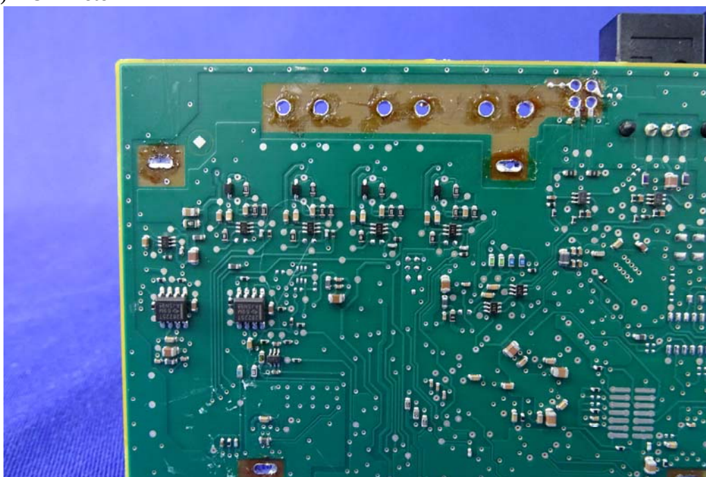
(25) EUT Photo
