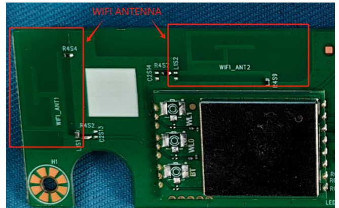
Wi-Fi Antenna
