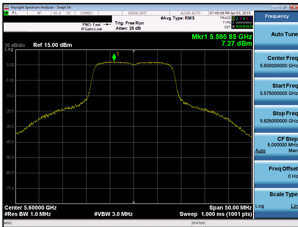
Plot 7-58. Power Spectral Density Plot (802.11a (UNII Band 2C) – Ch. 120)
