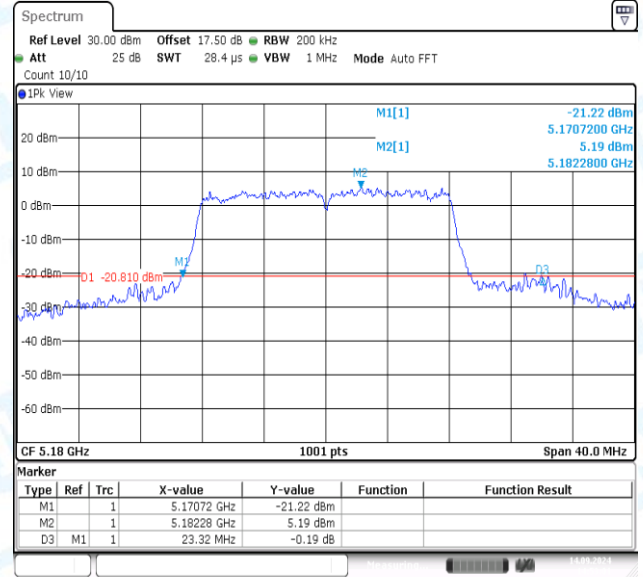
11A-Ant2-5180
