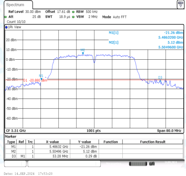
11N40MIMO-Ant2-5510
