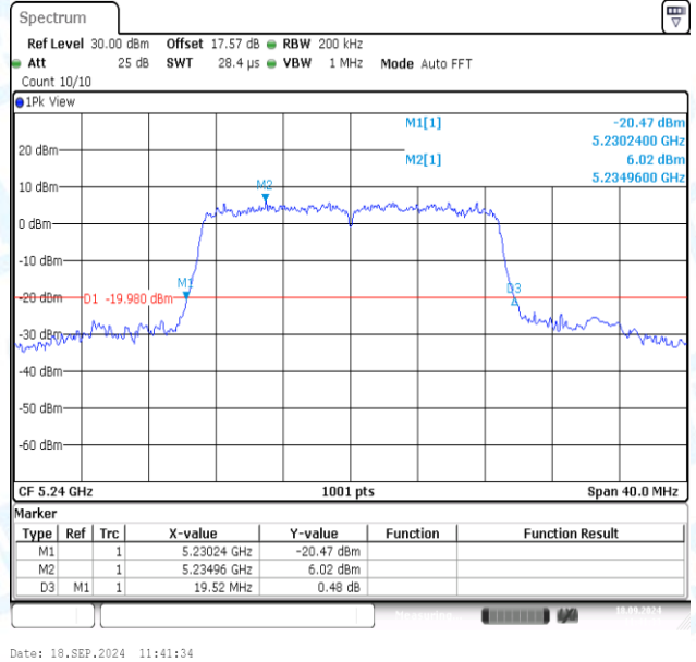
11AC20MIMO-Ant2-5240
