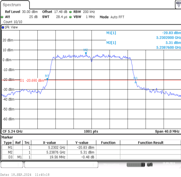
11AC20MIMO-Ant1-5240
