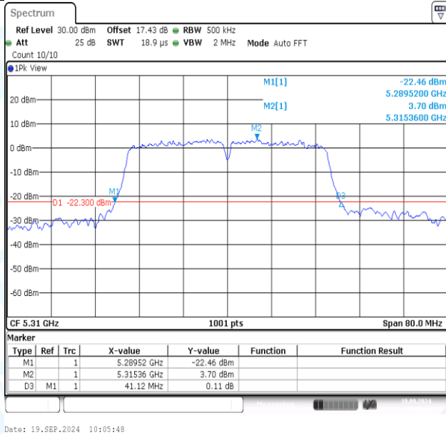
11AC40MIMO-Ant1-5310
