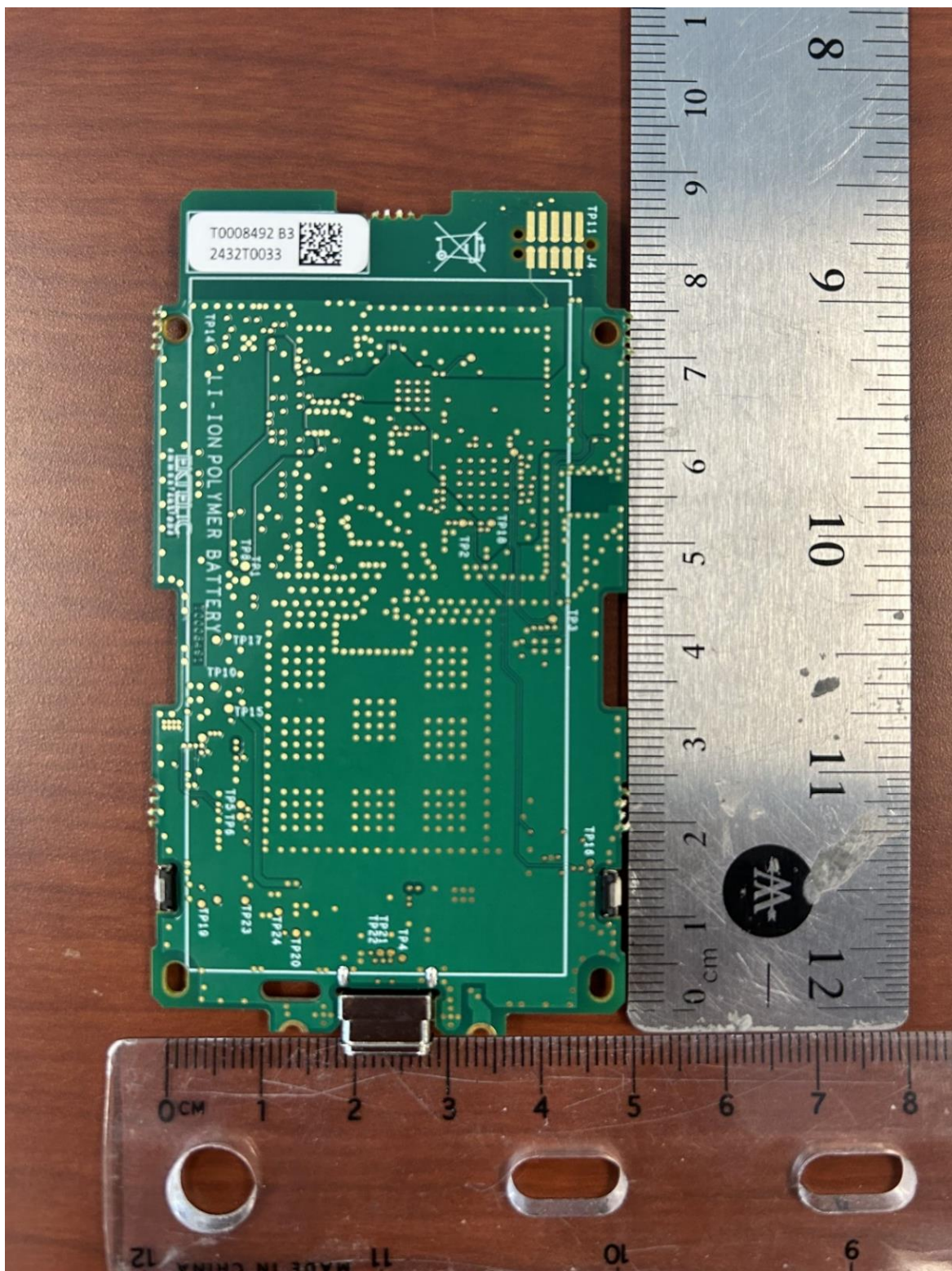
PCBA front view without battery (T0008534 / T0009142)
