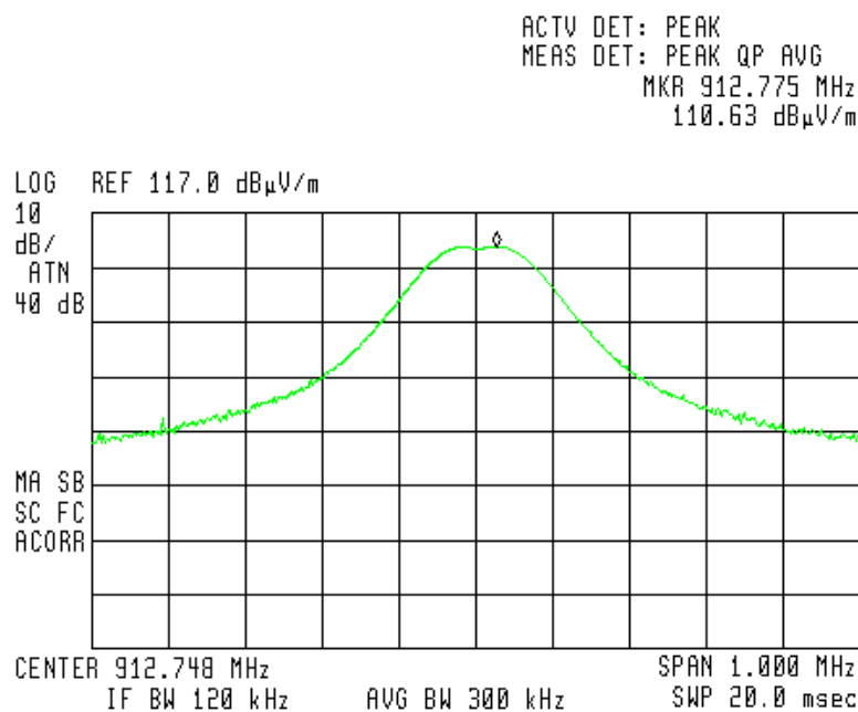
Figure 34 — 912.75 MHz-Horizontal – Wall Mounted
