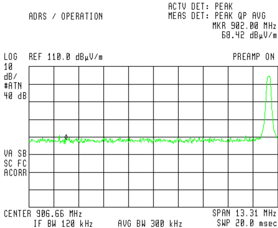
Figure 52 — 902.0 MHz Horizontal – Wall Mounted – Continuous Mode
