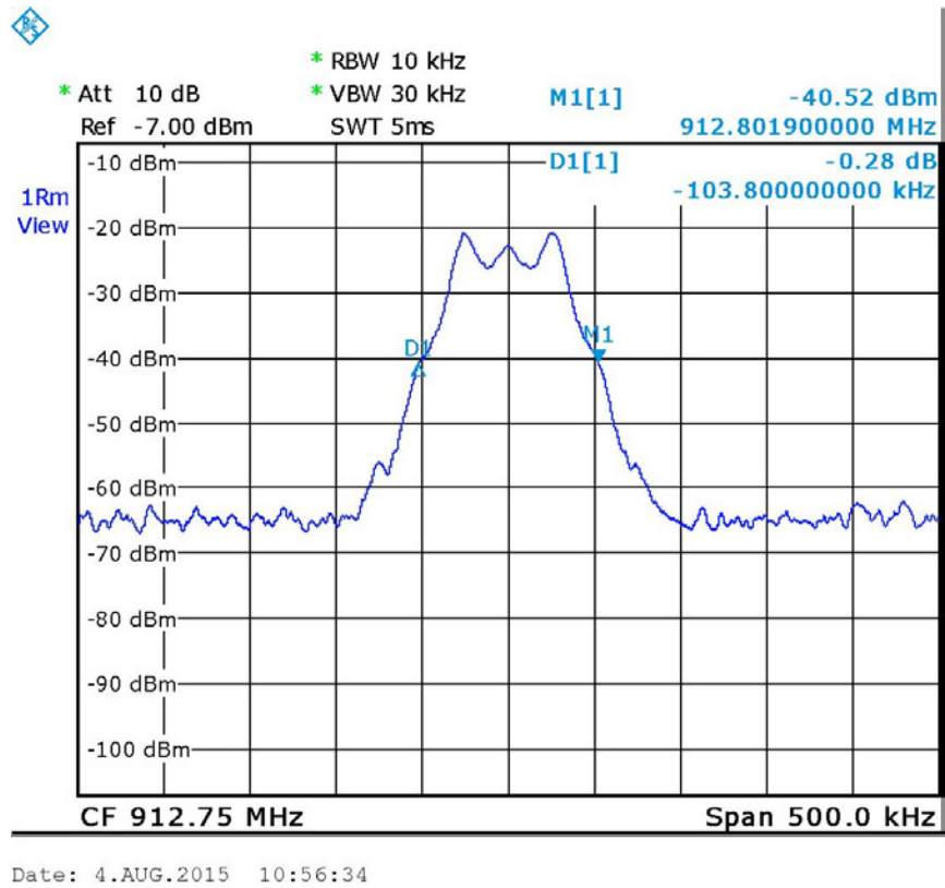
Figure 9. — 912.75 MHz
