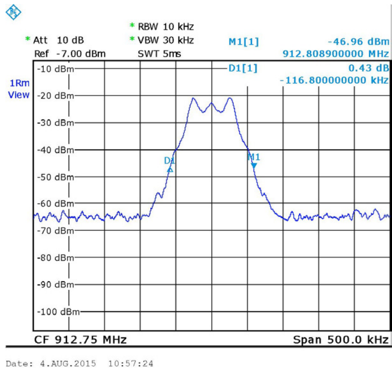
Figure 13. — 912.75 MHz
