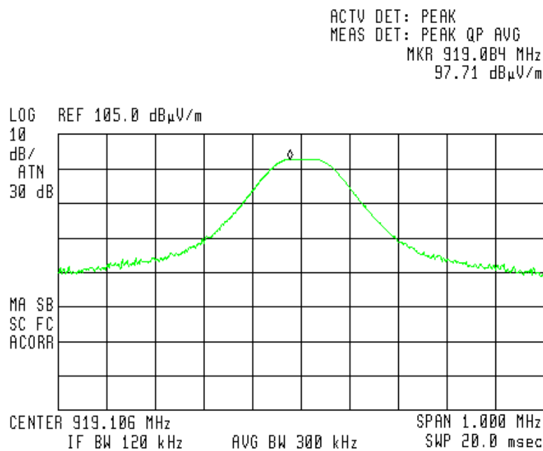
Figure 36 — 919.106 MHz Vertical – Wall Mounted
