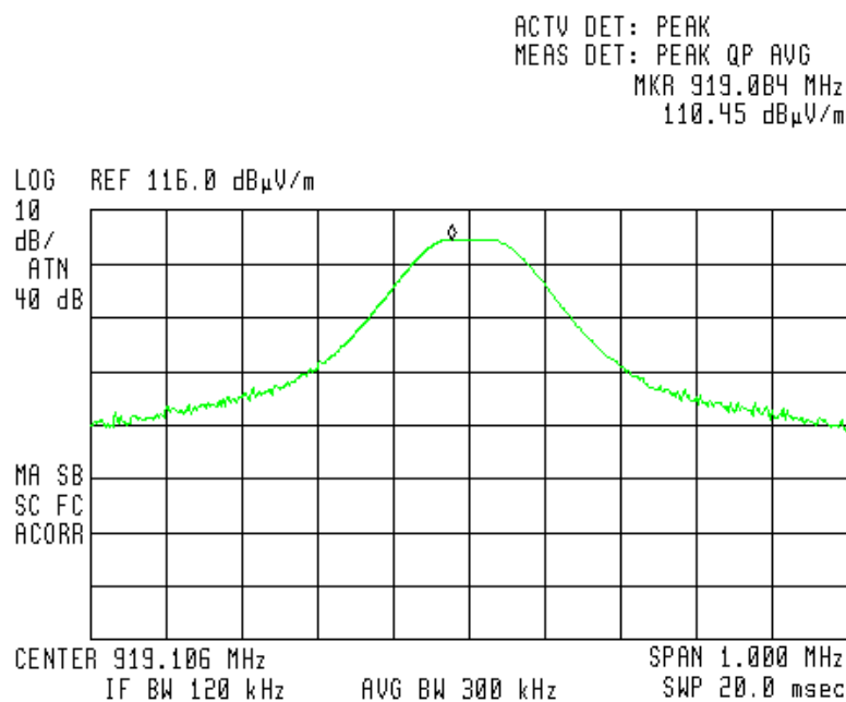
Figure 37 — 919.106 MHz Horizontal – Wall Mounted
