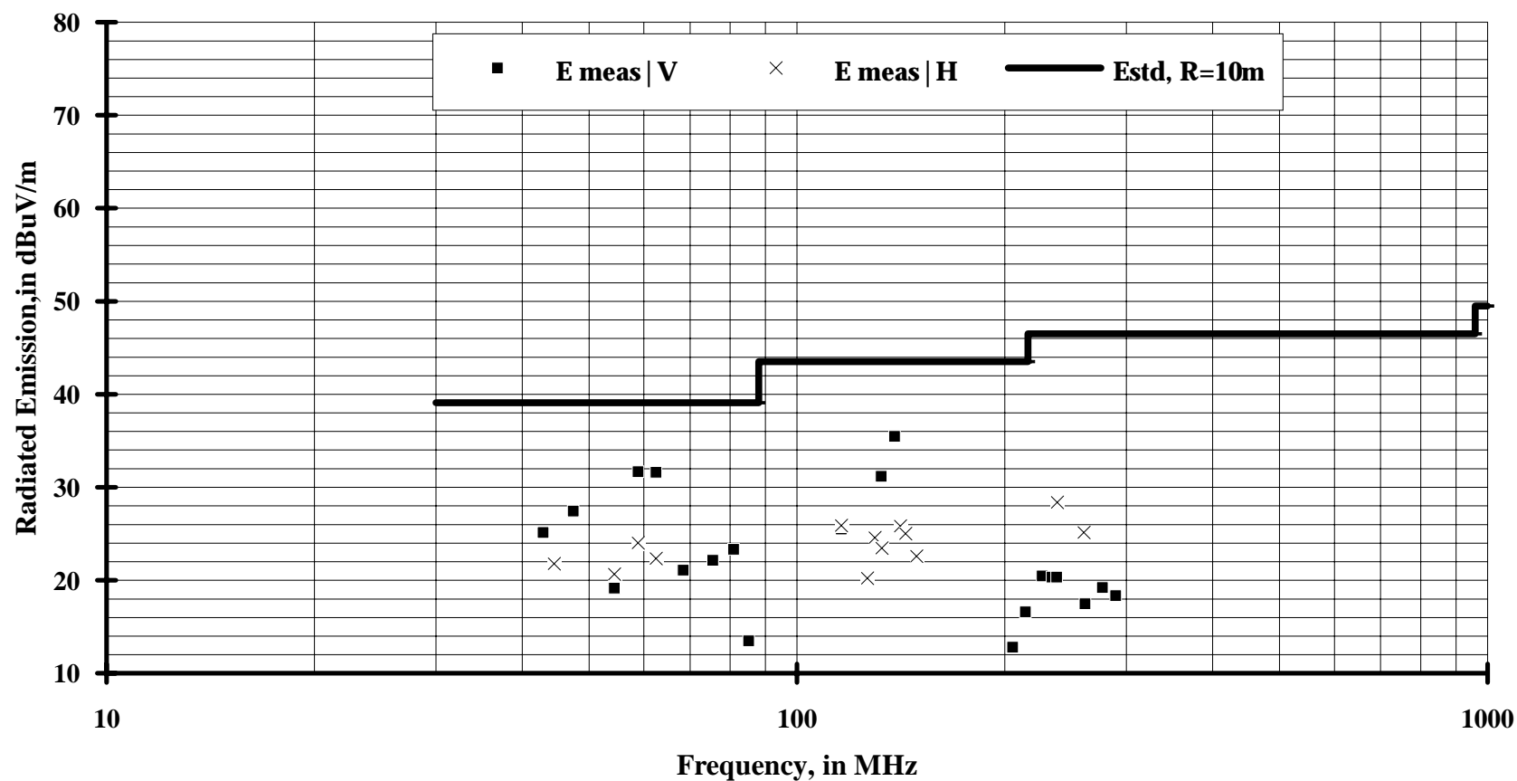
Fig.7 Radiated Emission vrs. FCC Class A Standard Limit, Vertical/Horizontal Polarization.
