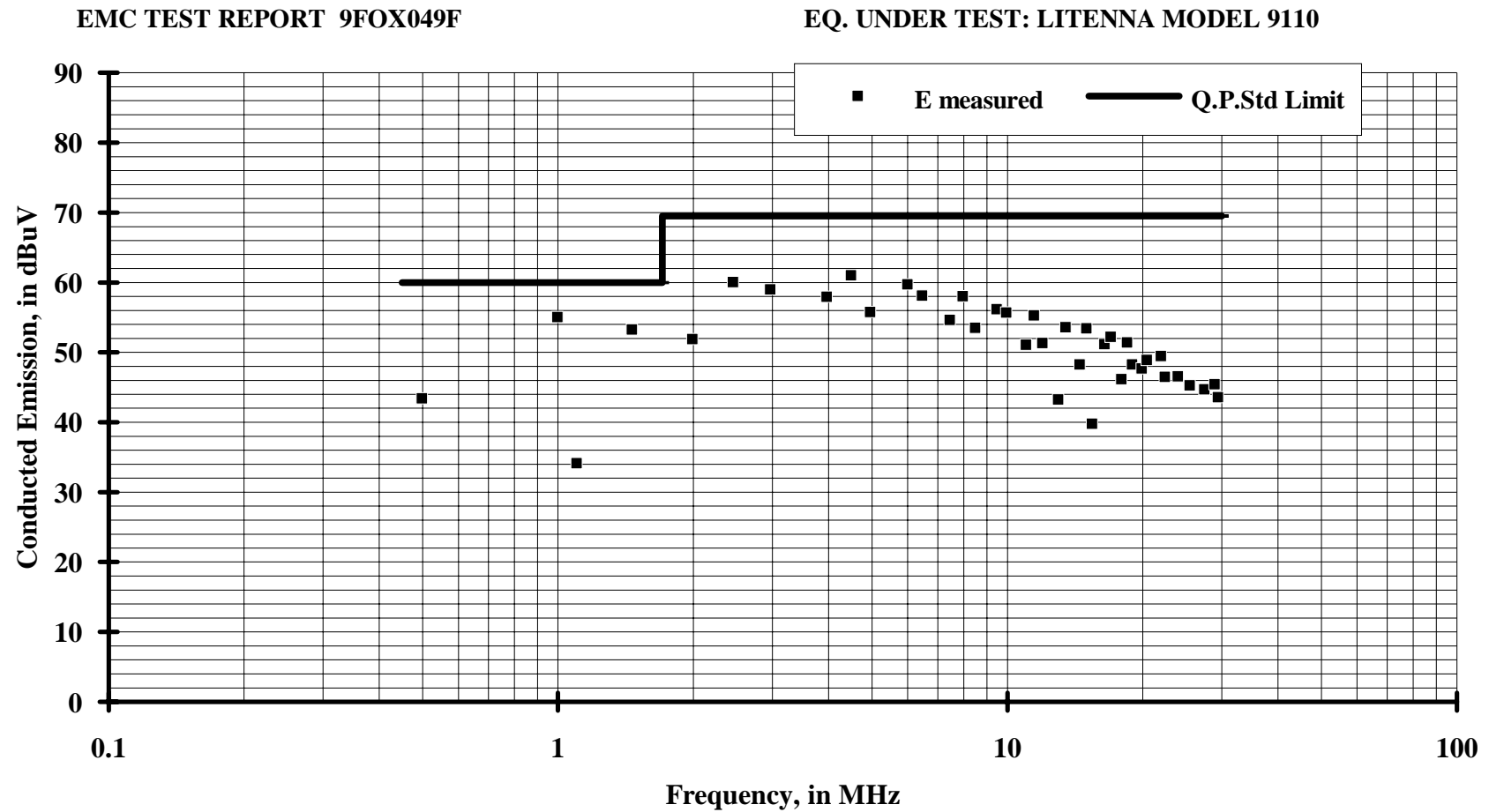
Fig. 5 Conducted Emission vrs. FCC Class A Standard Limit, DC Power Leads of Remote HUB Unit, +48VDC Lead, Q.P. Detector.
