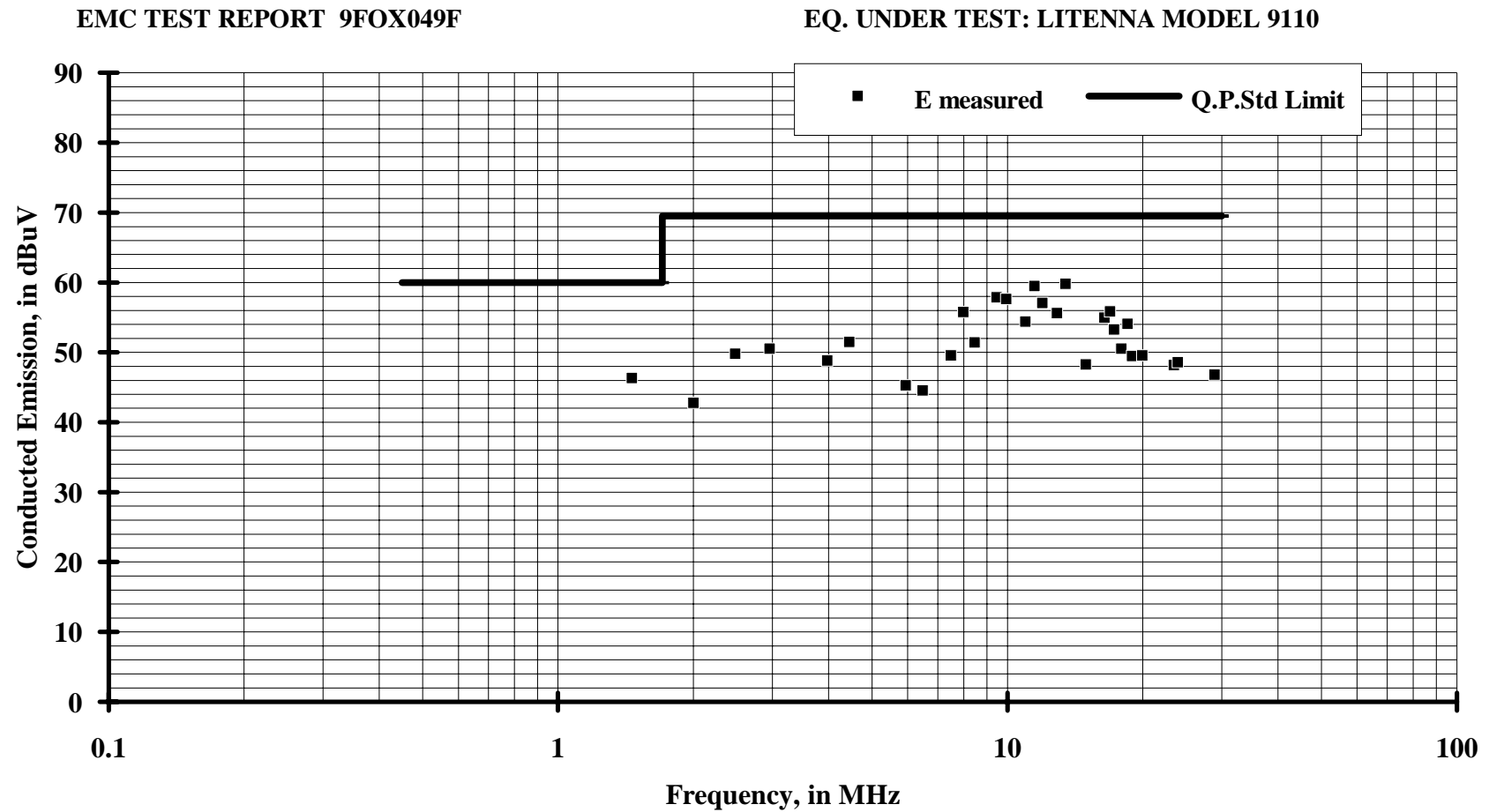
Fig. 2 Conducted Emission vrs. FCC Class A Standard Limit, AC Power Leads of AC/DC Power Supply, Neutral Lead, Q.P. Detector.
