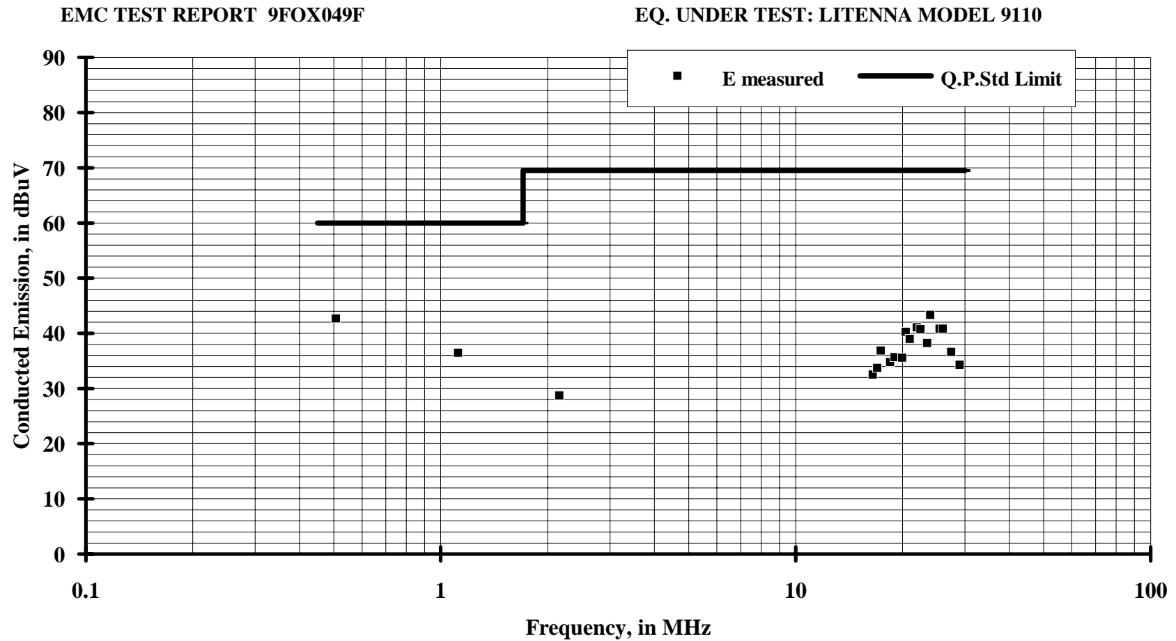
Fig. 3 Conducted Emission vrs. FCC Class A Standard Limit, DC Power Leads of Base Unit, +48VDC Lead, Q.P. Detector.
