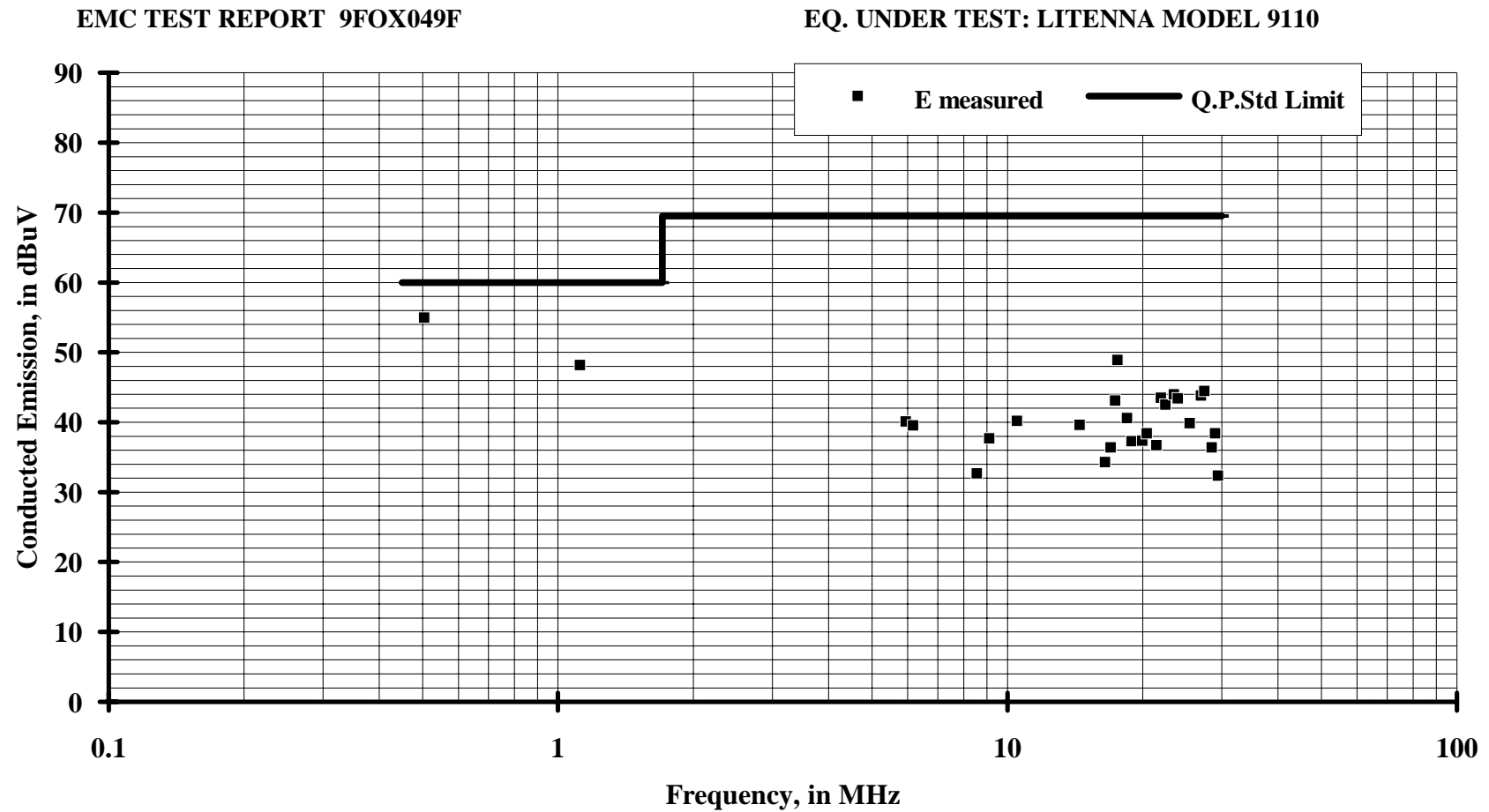
Fig. 4 Conducted Emission vrs. FCC Class A Standard Limit, DC Power Leads of Base Unit, 48V_RTN Lead, Q.P. Detector.
