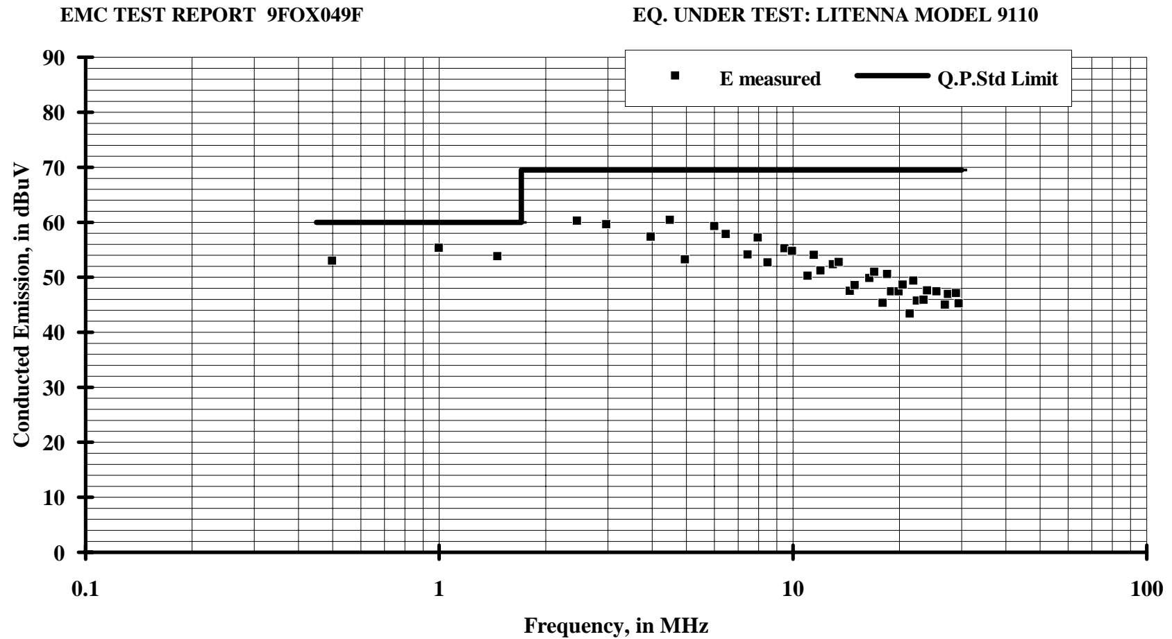
Fig. 6 Conducted Emission vrs. FCC Class A Standard Limit, DC Power Leads of Remote HUB Unit, 48V_RTN Lead, Q.P. Detector.
