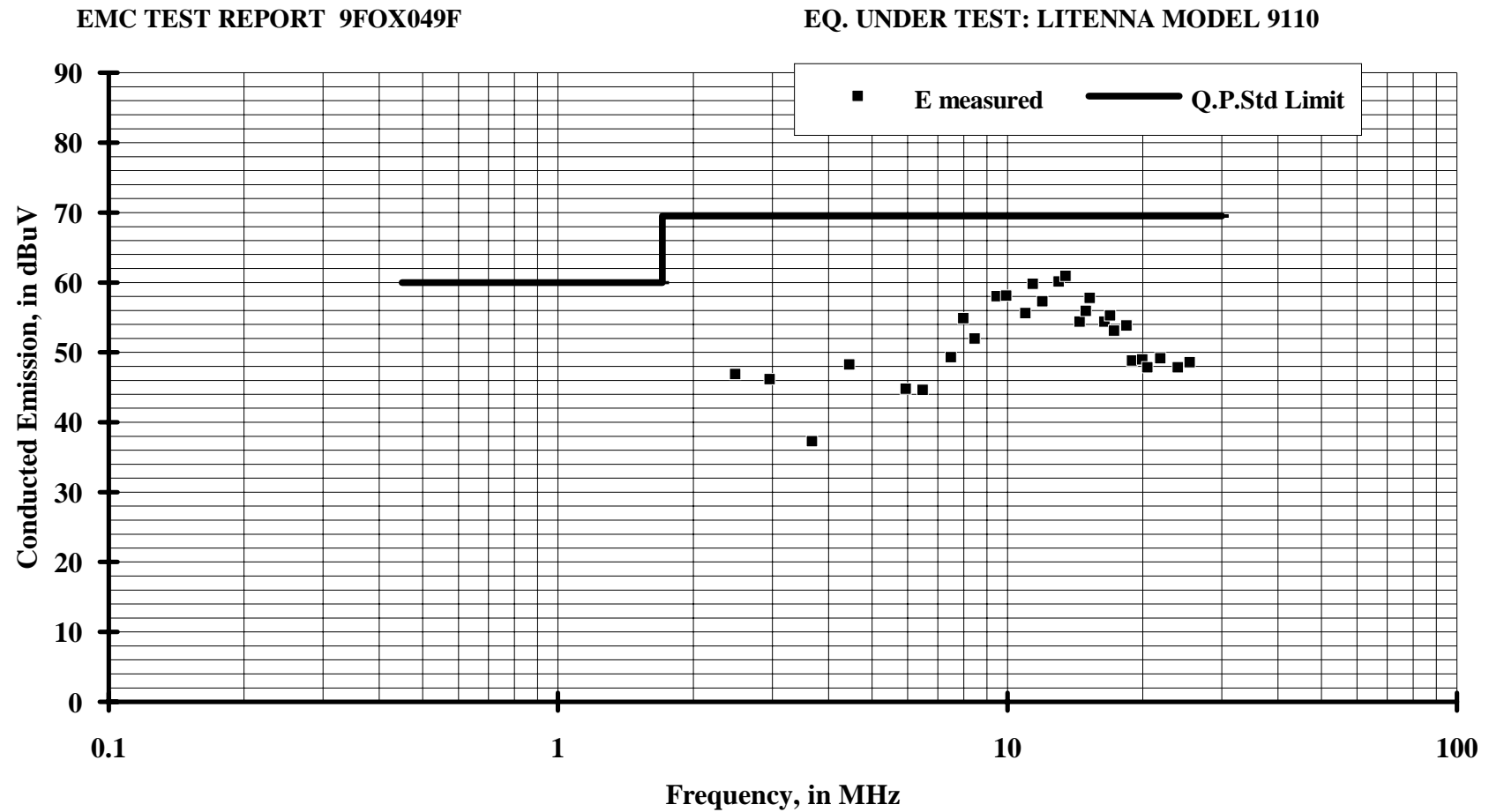
Fig. 1 Conducted Emission vrs. FCC Class A Standard Limit, AC Power Leads of AC/DC Power Supply, Phase Lead, Q.P. Detector.
