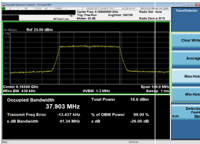
Plot 7-143. 26dB & 99% Bandwidth Plot Antenna 2a (40MHz 802.11ax (UNII Band 5) – Ch. 43, MCS4)
