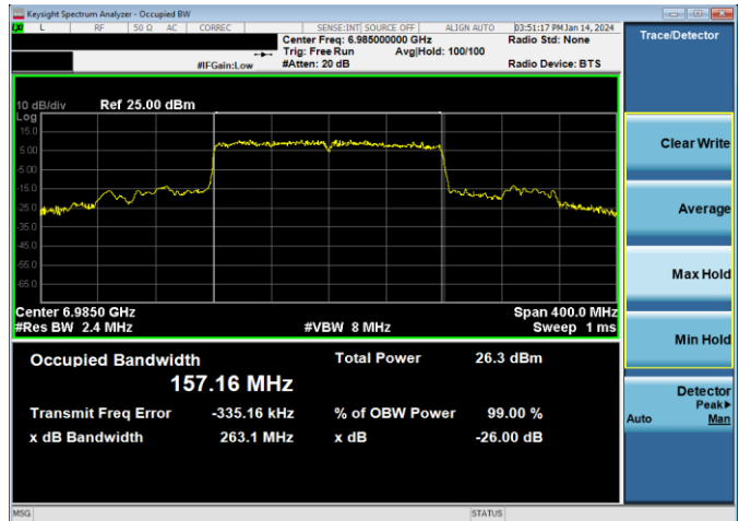
Plot 7-180. 26dB & 99% Bandwidth Plot Antenna 2a (160MHz 802.11ax (UNII Band 8) – Ch. 207, MCS11)
