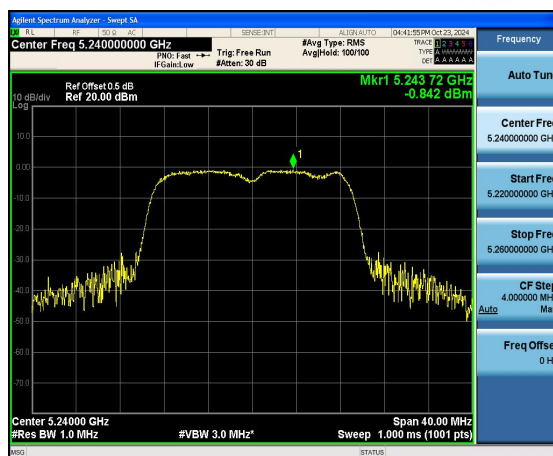
(802.11n20) PSD plot on channel 48
