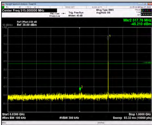
Band12-1.4MHz-16QAM-23173-1RB#0-Range1:30~1000M Hz
