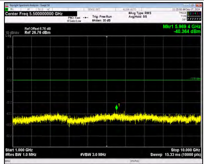
Band12-1.4MHz-QPSK-23173-1RB#0-Range2:1000~1000 OMHz
