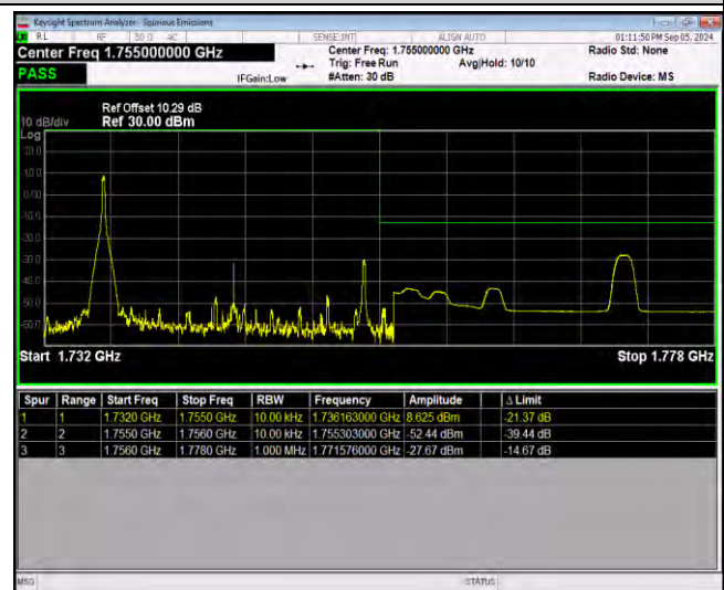
Band4-20MHz-16QAM-20300-27RB#0
