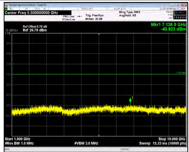
Band12-1.4MHz-16QAM-23173-1RB#0-Range2:1000~10000MHz
