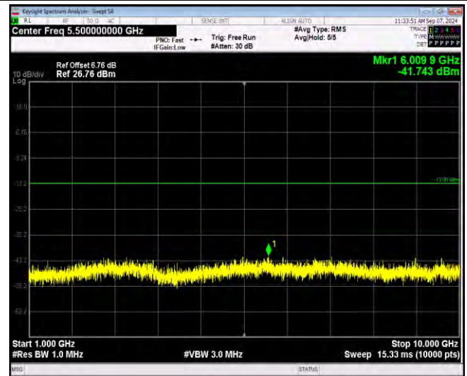
Band12-1.4MHz-QPSK-23095-1RB#0-Range2:1000~1000 OMHz
