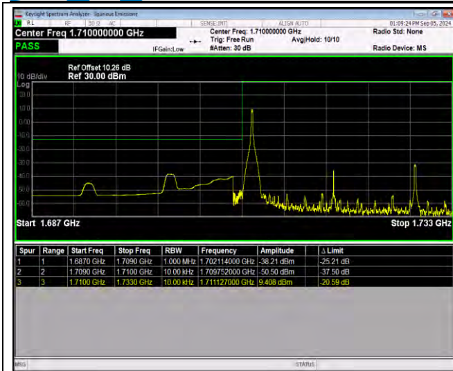
Band4-20MHz-16QAM-20050-27RB#0
