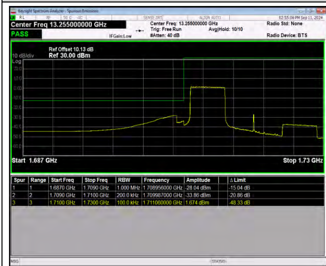
Band4-20MHz-16QAM-20300-1RB#99
