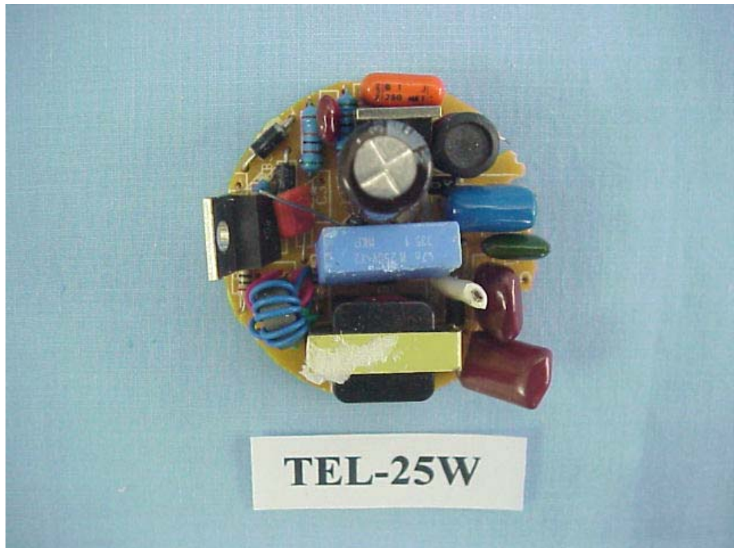
FIGURE 11 ENERGY SAVING LAMP (M/N: TEL-25W) MAIN BOARD (COMPONENT SIDE)
