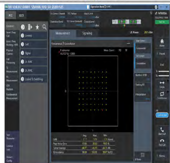
1-N25--15-40-M-4-DFT-64QAM-Outter_Full-216@0- Ant1-see graph-PASS
