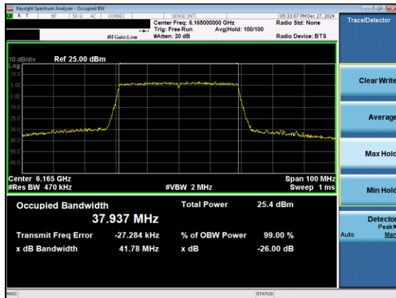
Plot 7-2. 26dB & 99% Bandwidth Plot Antenna 5T (40MHz 802.11ax (UNII Band 5) – Ch. 43)
