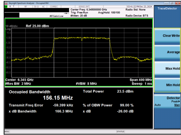
Plot 7-16. 26dB & 99% Bandwidth Plot Antenna 5T (160MHz 802.11ax (UNII Band 5) – Ch. 79)
