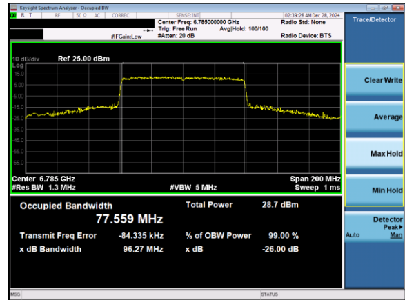
Plot 7-39. 26dB & 99% Bandwidth Plot Antenna 3b (80MHz 802.11ax (UNII Band 7) – Ch. 167)
