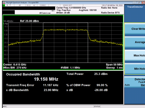
Plot 7-29. 26dB & 99% Bandwidth Plot Antenna 3b (20MHz 802.11ax (UNII Band 5) – Ch. 93)
