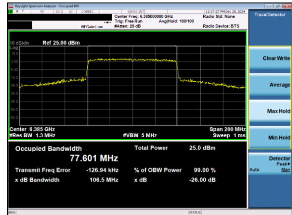
Plot 7-59. 26dB & 99% Bandwidth Plot Antenna 1b (80MHz 802.11ax (UNII Band 5) – Ch. 87)
