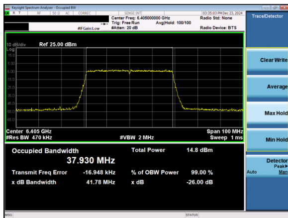
Plot 7-14. 26dB & 99% Bandwidth Plot Antenna 5T (40MHz 802.11ax (UNII Band 5) – Ch. 91)
