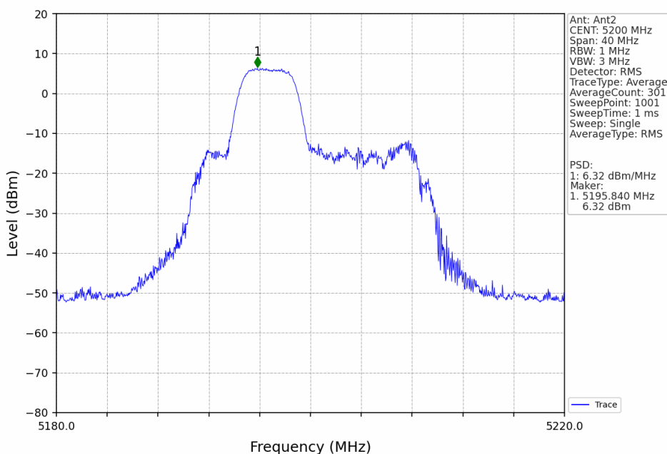
802.11ax(HEW20)_MCH_5200MHz_RU52_Mid_Ant2_NTNV
