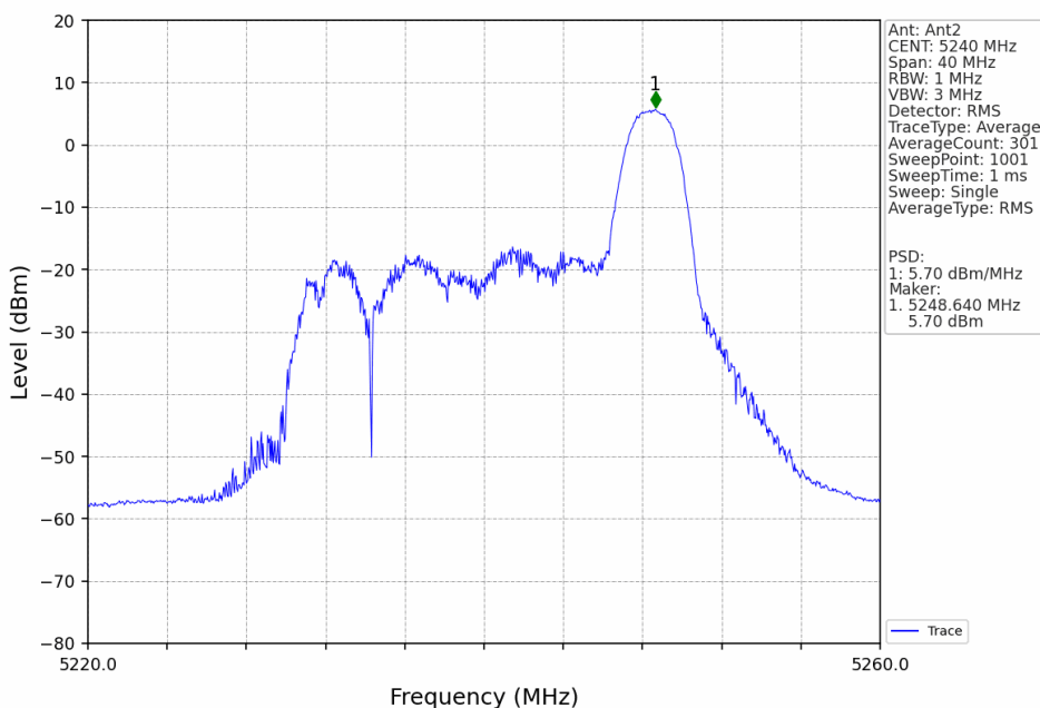
802.11ax(HEW20)_HCH_5240MHz_RU26_Right_MIMO_NTNV
