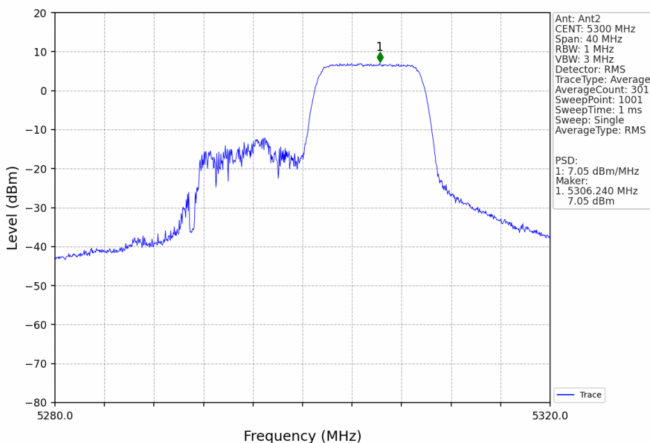
802.11ax(HEW20)_MCH_5300MHz_RU106_Right_MIMO_NTNV
