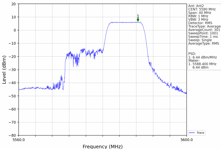
802.11ax(HEW20)_MCH_5580MHz_RU106_Right_MIMO_NTNV
