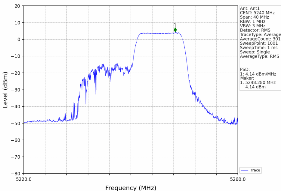
802.11ax(HEW20)_HCH_5240MHz_RU106_Right_Ant1_NTNV
