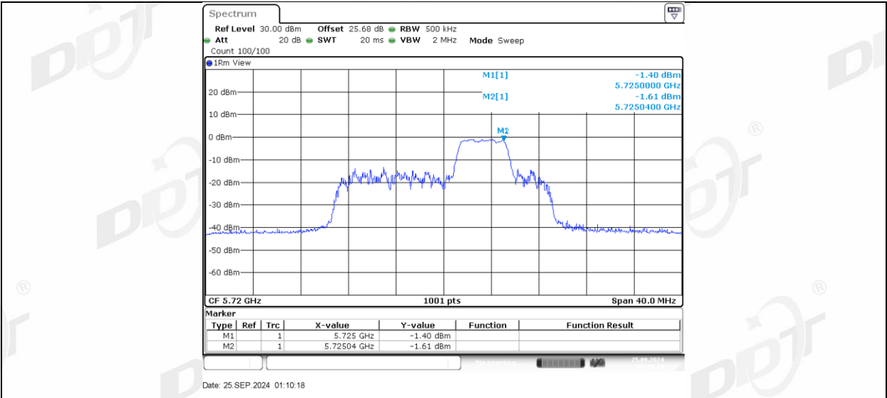
11AX20MIMO Ant2 5720 UNII-3 52Tone RU40
