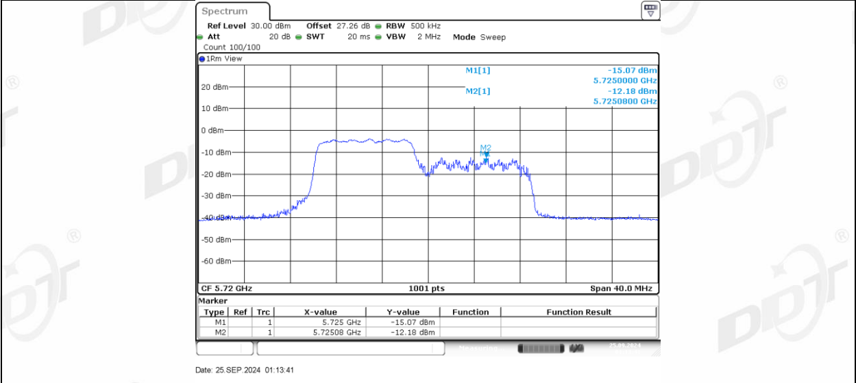
11AX20MIMO Ant2 5720 UNII-3 106Tone RU54
