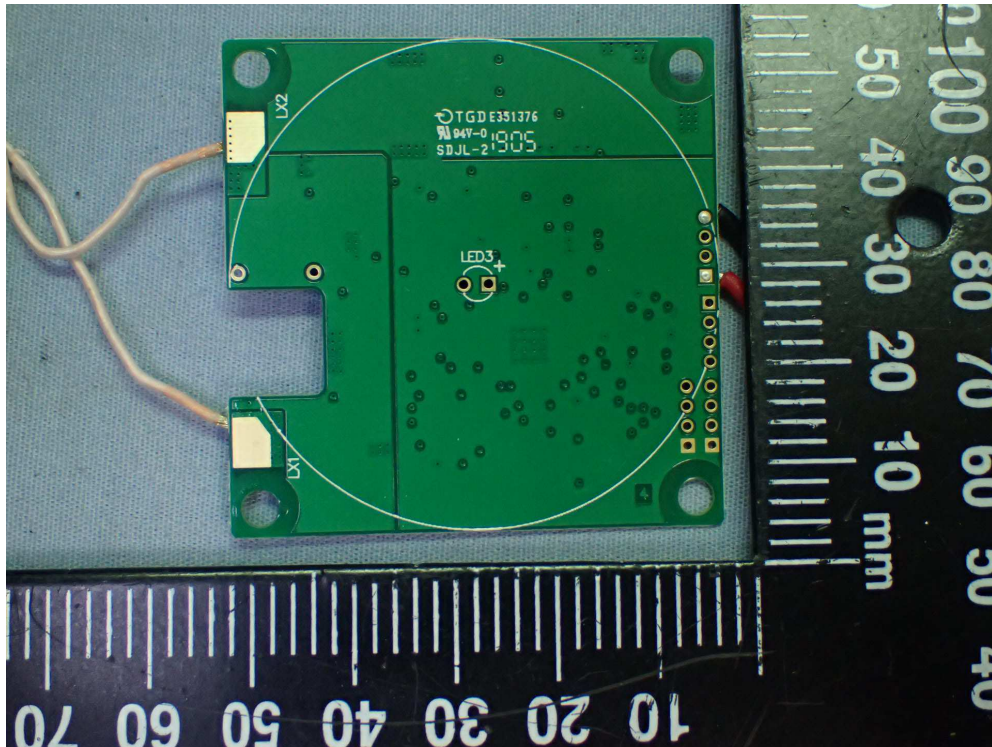
Figure 3 General Appearance (Back View)
