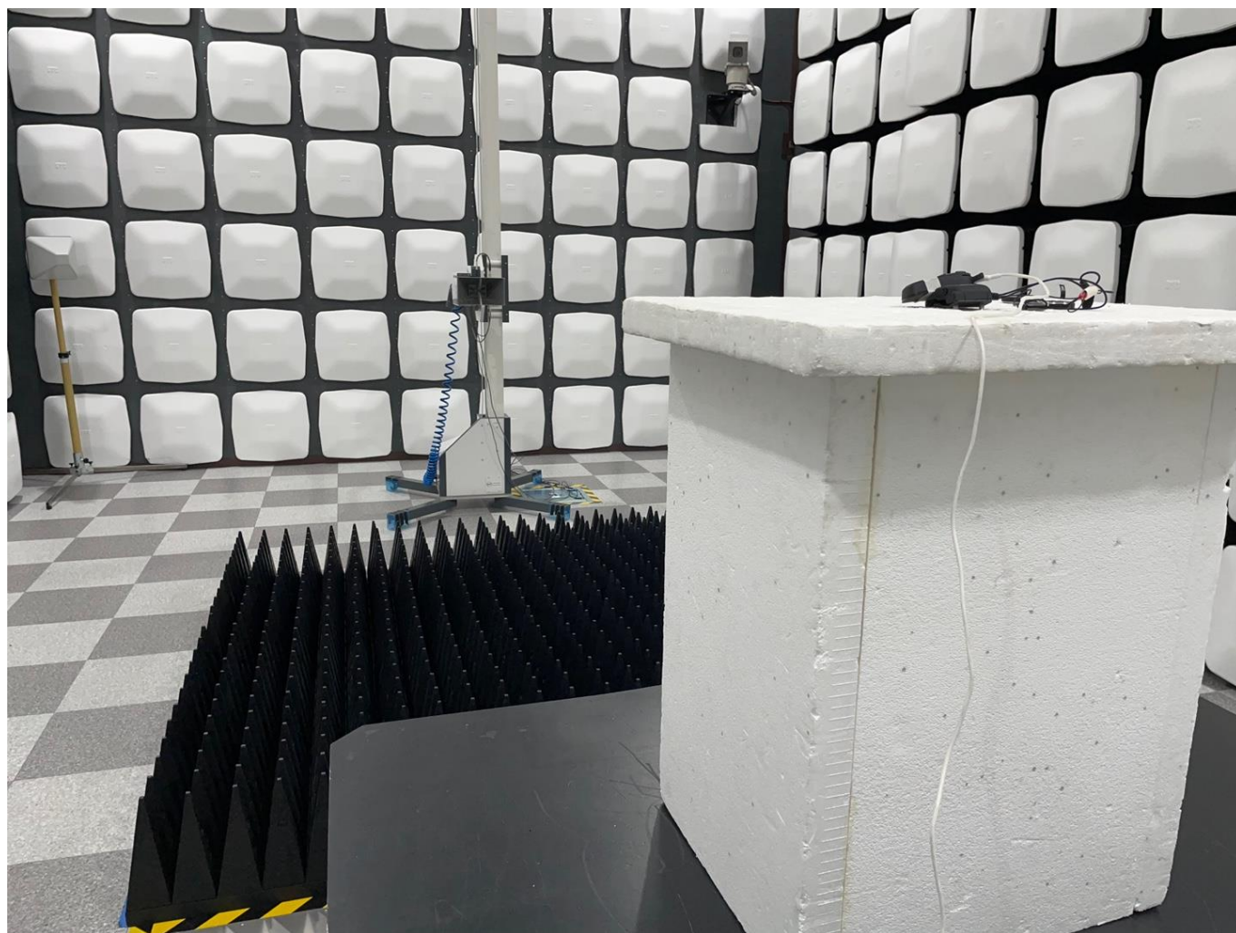
Above 1 GHz
