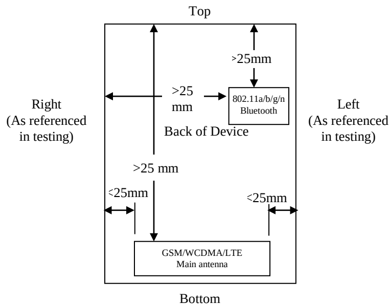
Figure 1.8.2-1 Identification of all sides for SAR Testing
