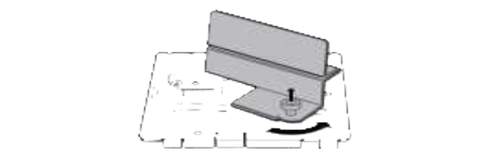
Figure 3 Attaching the adapter to the main bracket
