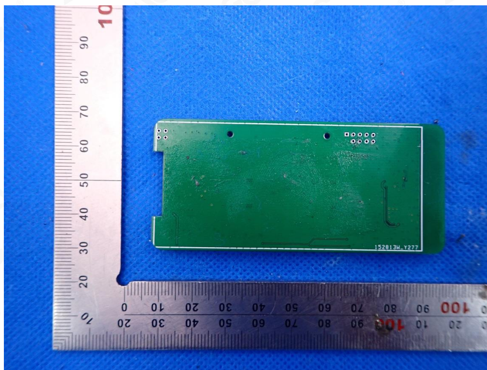
INTERNAL VIEW-3 OF EUT(KESL042C)
