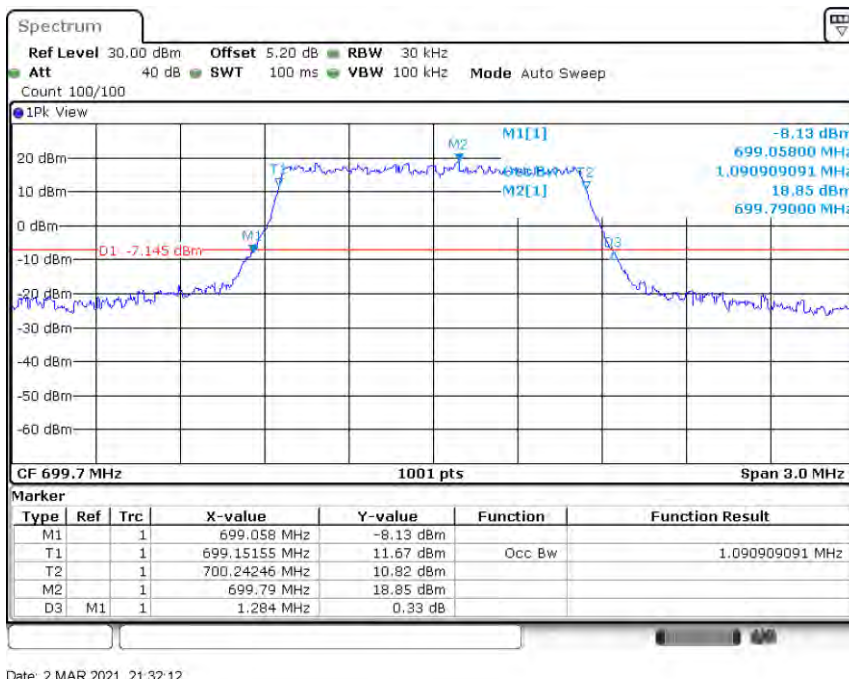
Band12-1.4MHz-QPSK-23095-6RB#0-1.091
