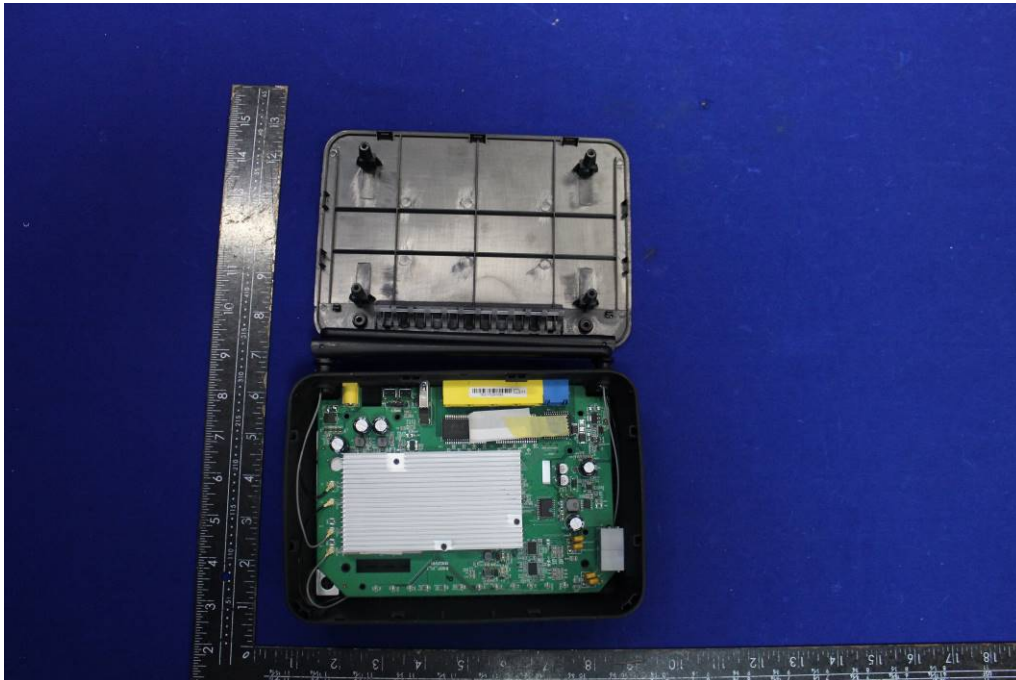
EUT Housing and Board View 1
