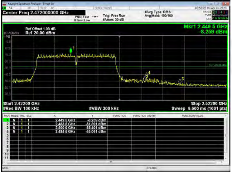
Highest channel
