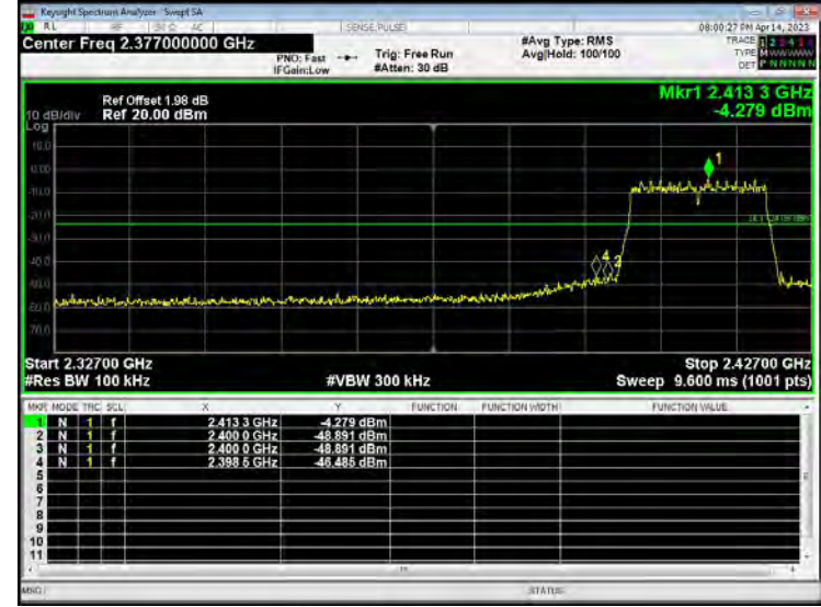
Lowest channel
