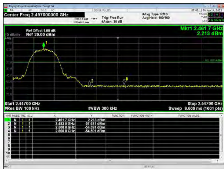
Highest channel
