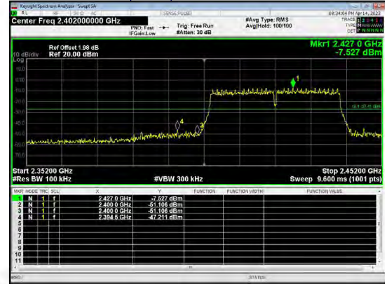
Lowest channel
