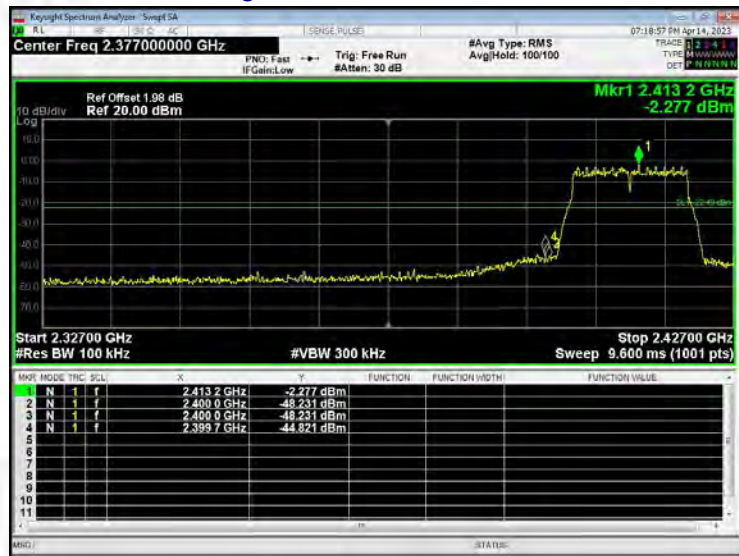
Lowest channel
