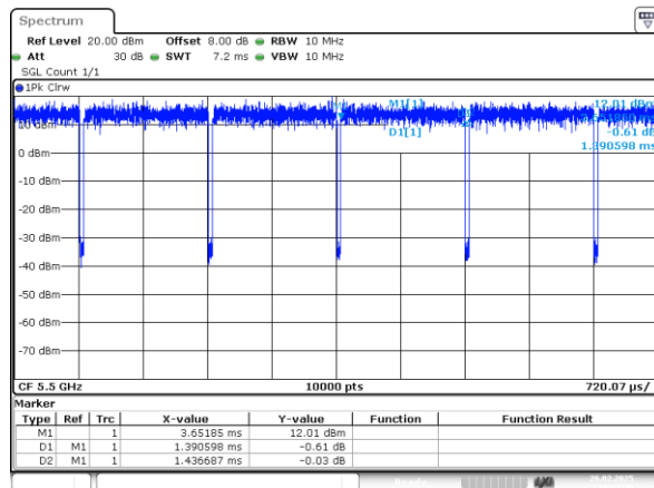
802.11a_5500MHz_Chain 0
