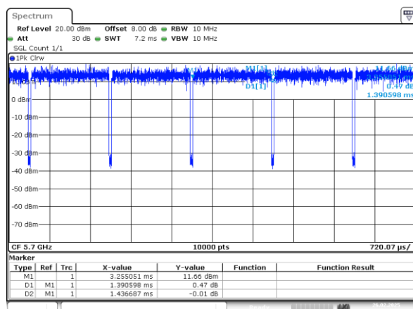
802.11a_5700MHz_Chain 0
