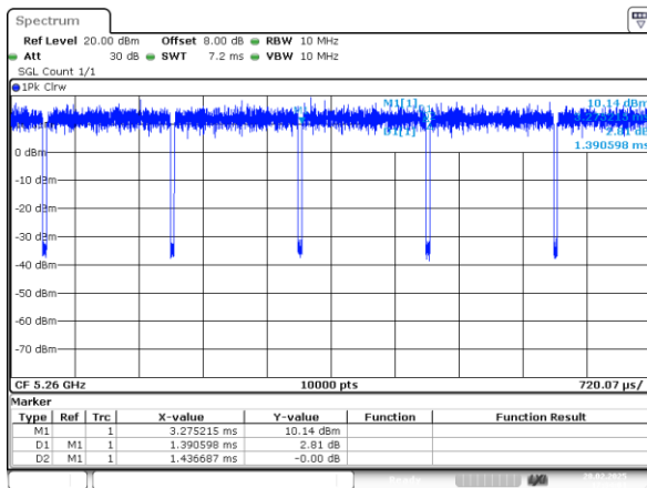
802.11a_5260MHz_Chain 0
