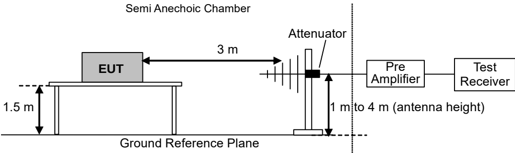
Figure 2: Test Setup
