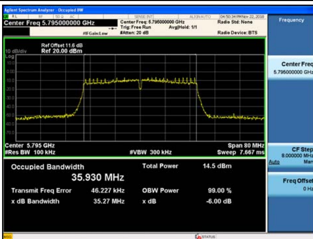
802.11ac(VHT40) (CH.159)
