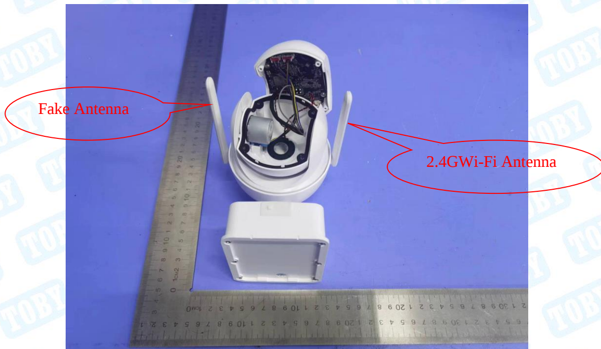
Photo 12 Internal of EUT
