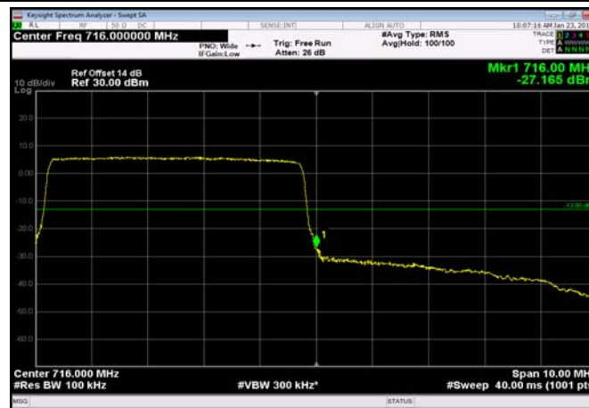
HighRange_FDD17_10MHz_711_OneRB _high_Q16
