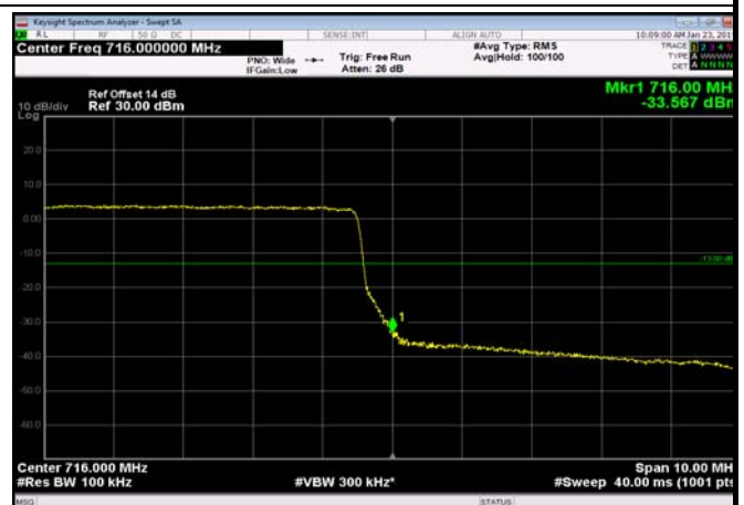
HighRange_FDD17_10MHz_711_fullRB _High_QPSK
