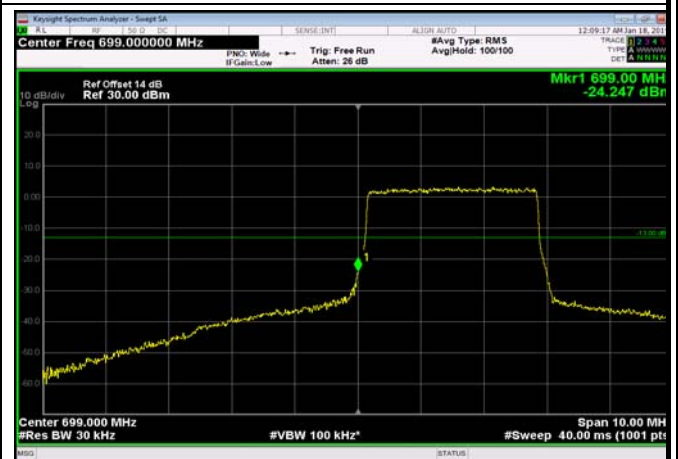
LowRange_FDD12_5MHz_701.5_OneRB _low_Q16
