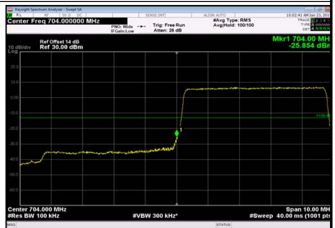
LowRange_FDD17_10MHz_709_OneRB _low_QPSK
