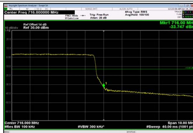
HighRange_FDD17_10MHz_711_fullRB _High_Q16
