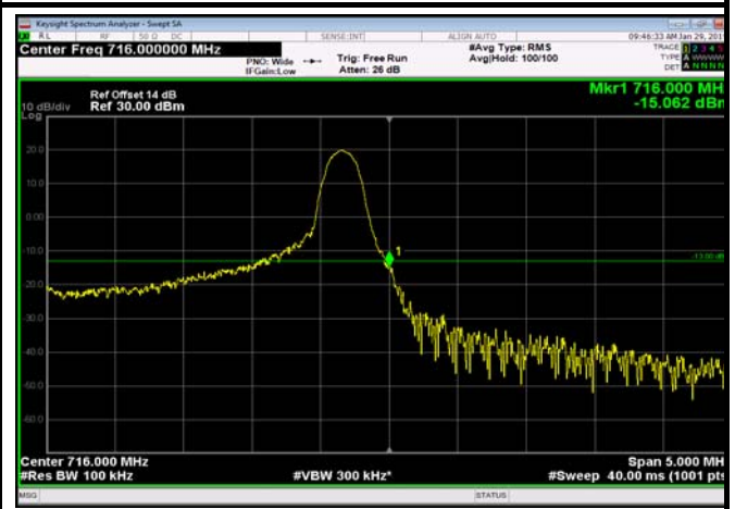
HighRange_FDD17_5MHz_713.5_OneRB _high_Q16
