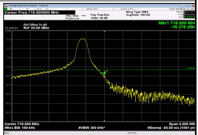
HighRange_FDD17_5MHz_713.5_OneRB _high_QPSK
