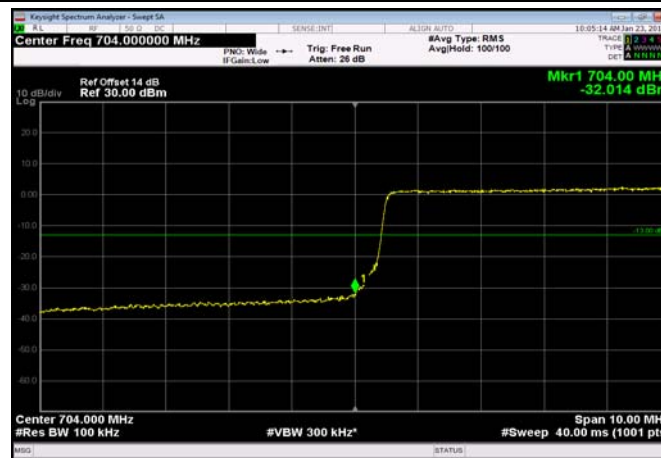
LowRange_FDD17_5MHz_706.5_fullRB _Low_Q16
