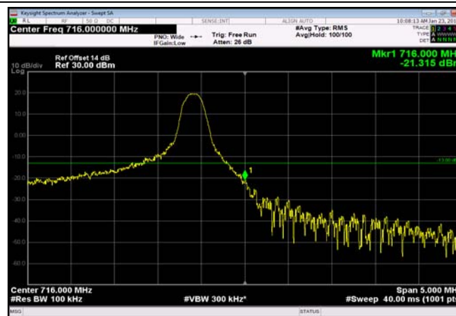
HighRange_FDD17_5MHz_713.5_OneRB _high_Q16
