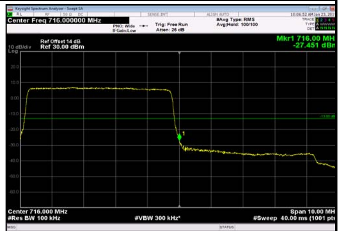
HighRange_FDD17_10MHz_711_OneRB _high_QPSK
