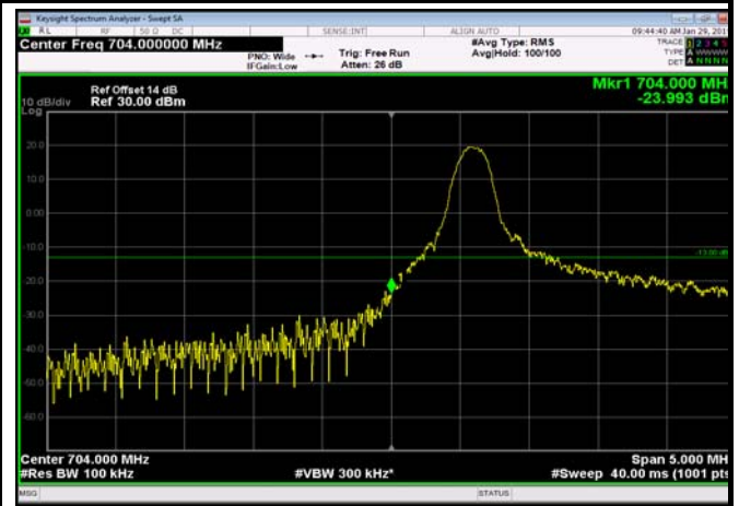
LowRange_FDD17_10MHz_709_fullRB _Low_Q16
