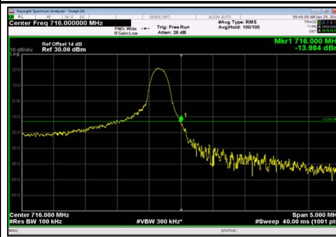
HighRange_FDD17_5MHz_713.5_OneRB _high_QPSK
