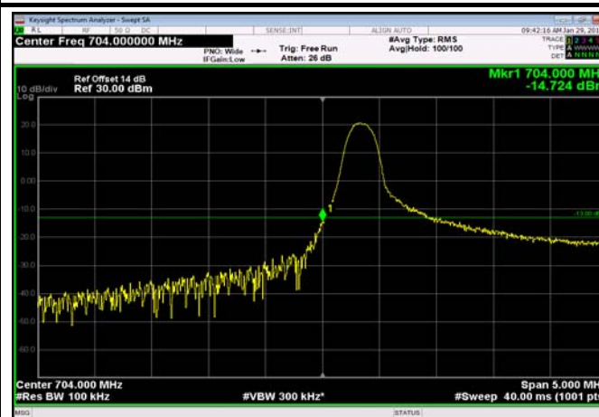
LowRange_FDD17_5MHz_706.5_fullRB _Low_QPSK
