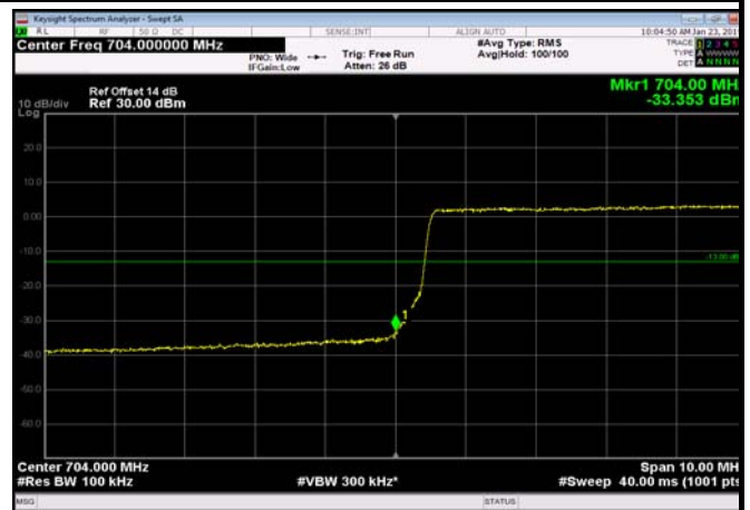
LowRange_FDD17_5MHz_706.5_fullRB _Low_QPSK
