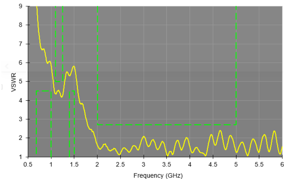
VSWR ANT3(DG)
