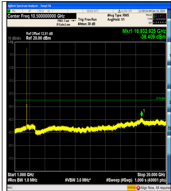
Band7_10MHz_16QAM_20800_50RB#0_1000~ 20000_1000~20000
