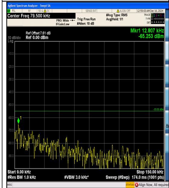
Band7_10MHz_16QAM_21100_50RB#0_0.009~ 0.15_0.009~0.15
