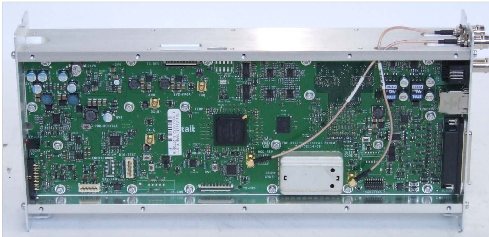
Photograph 04: Control PCB - Top
