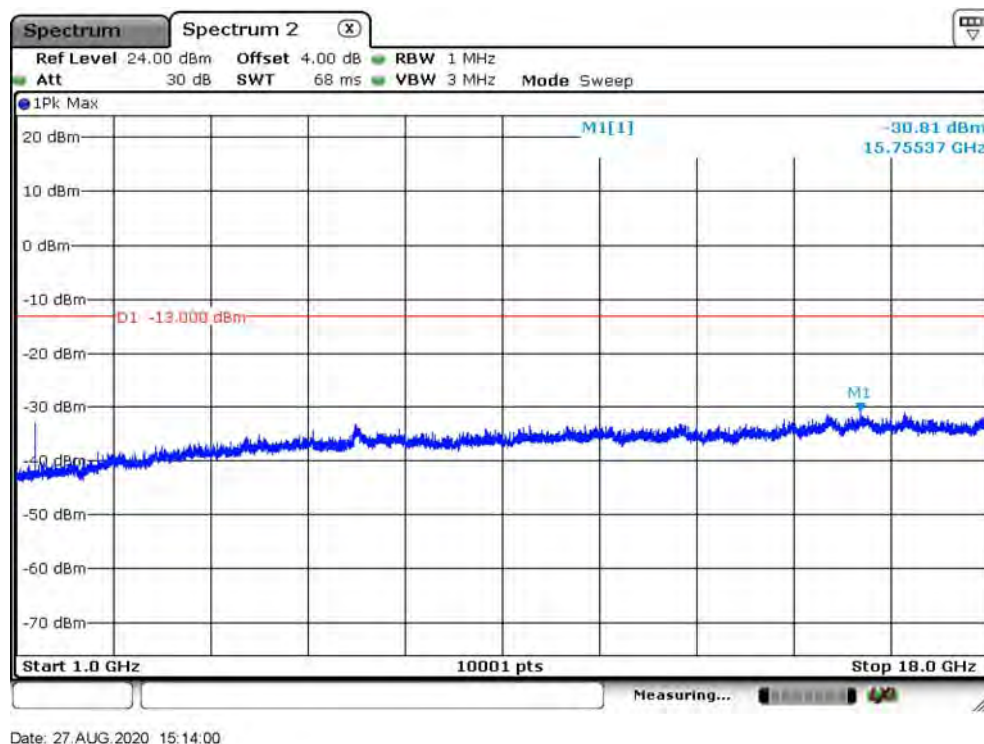
B71_CH133147_5M_1RB12_QPSK_Above 1G
