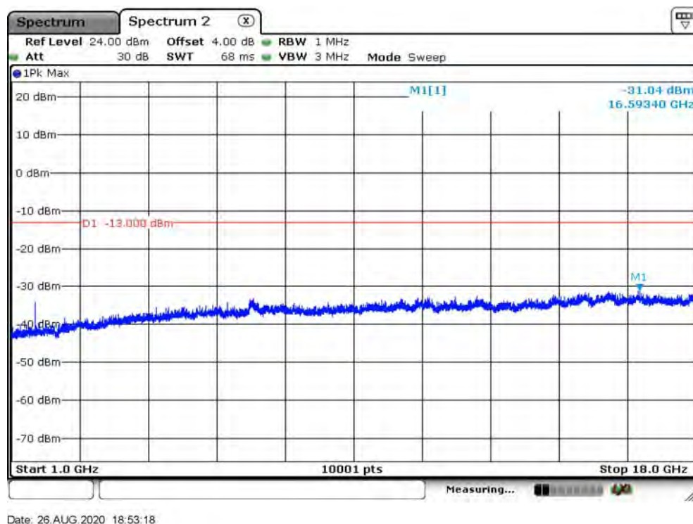
B14_CH23305_5M_1RB0_QPSK_Above 1G
