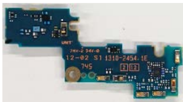
Internal Main_ANT-1-PWB (back-side)
