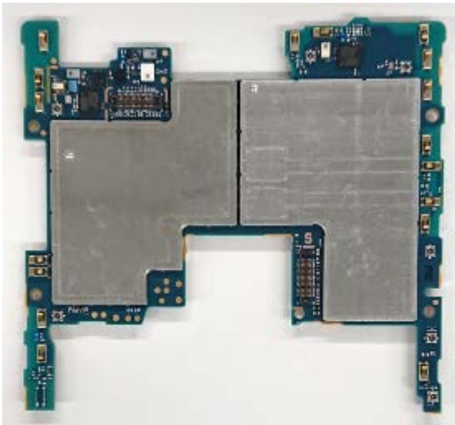
Internal PWB with Shield cases (Rear-side)
