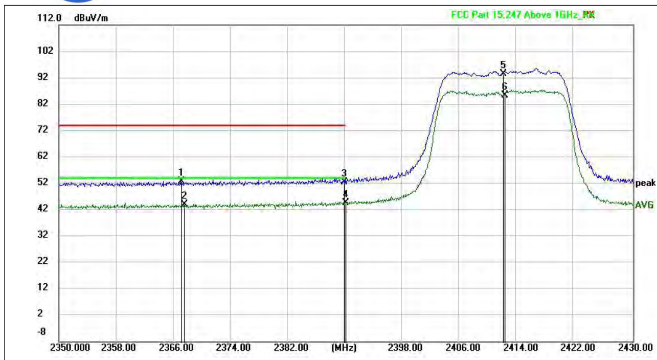
(802.11n_20M_2412MHz, Antenna Vertical)
