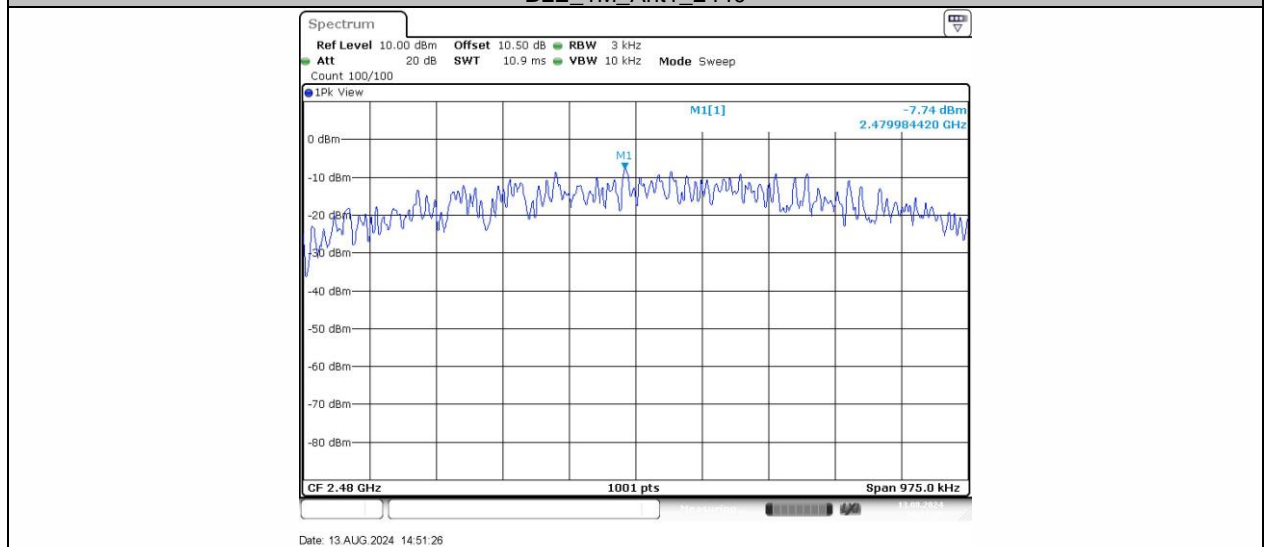
BLE_1M_Ant1_2480
