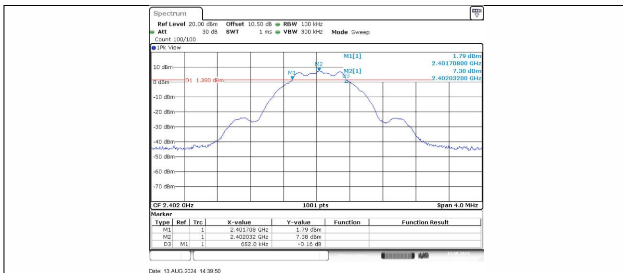
BLE_1M_Ant1_2402
