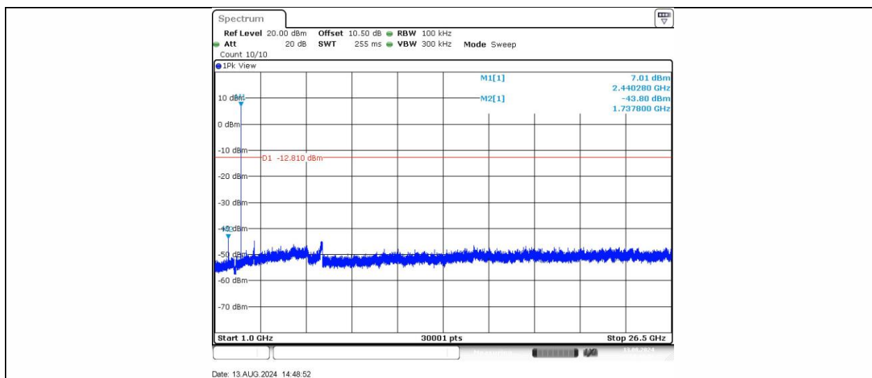
BLE_1M_Ant1_2440_1000-26500
