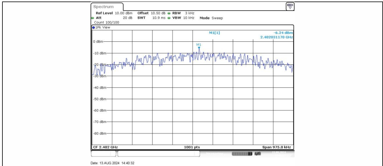
BLE_1M_Ant1_2402
