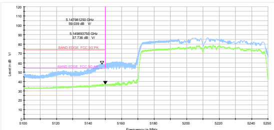
802.11ac VHT80-Channel 42: Peak+Average
