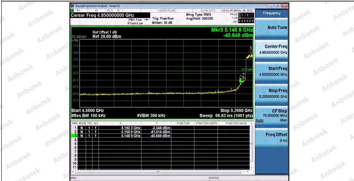
11N40SISO_Ant1_High_5230
