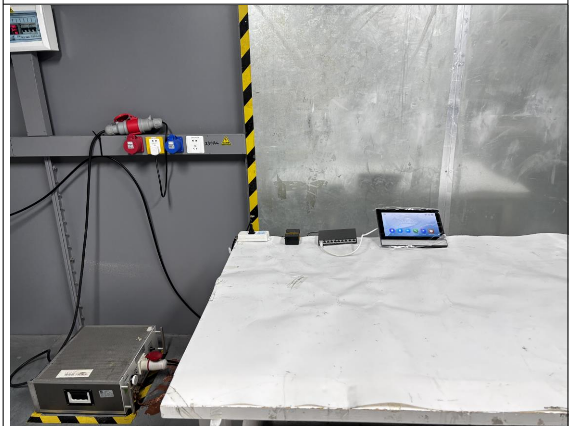
Conducted emission
