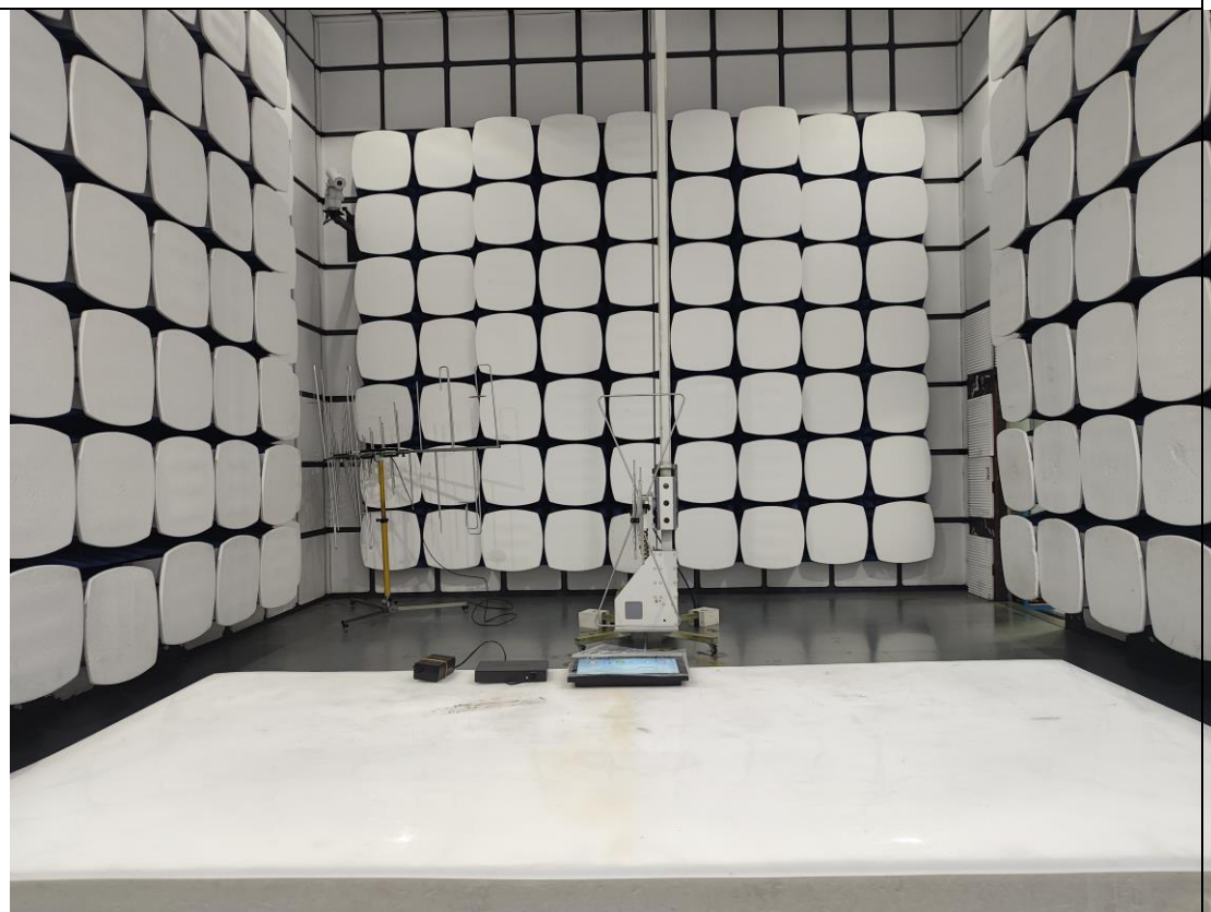
Radiated Emission
