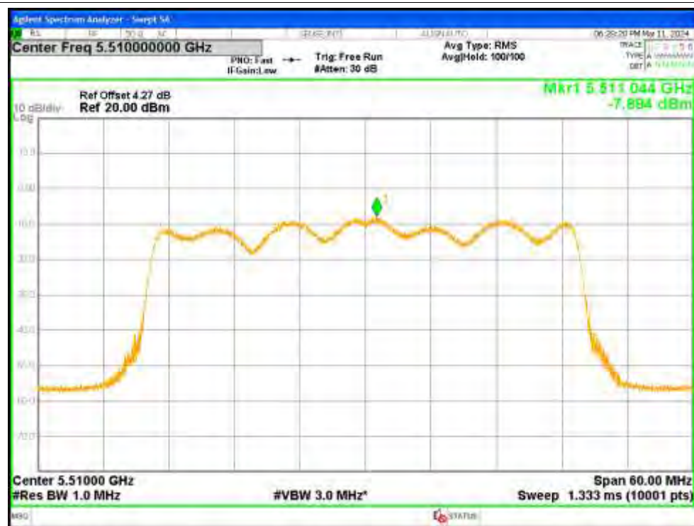
PSD NVNT ax40 5510MHz Ant4
