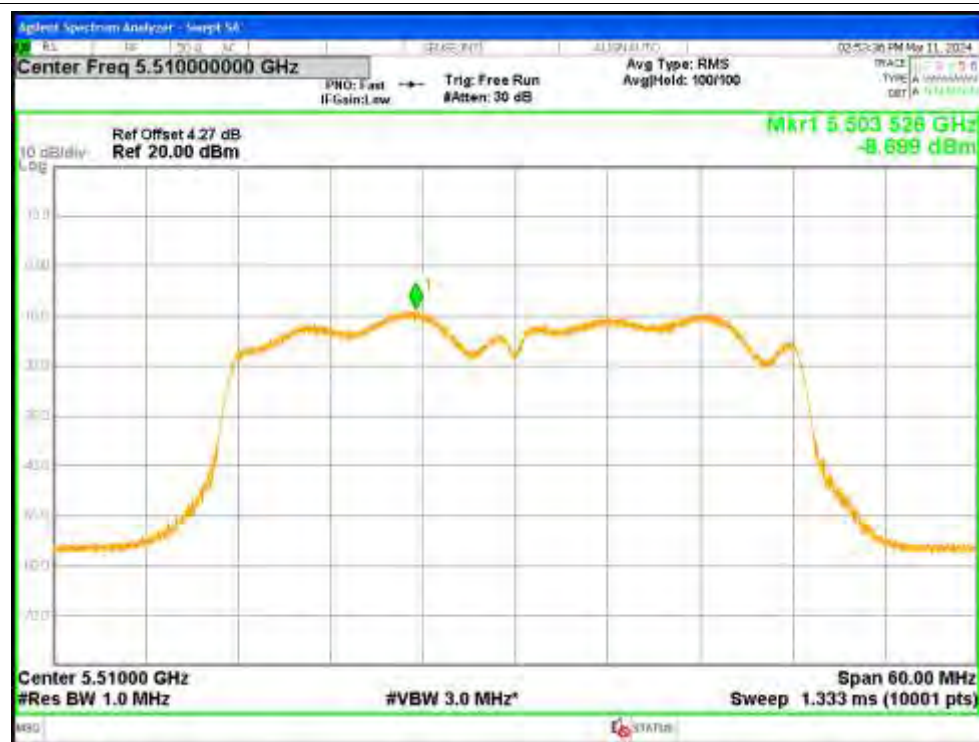
PSD NVNT ac40 5510MHz Ant4
