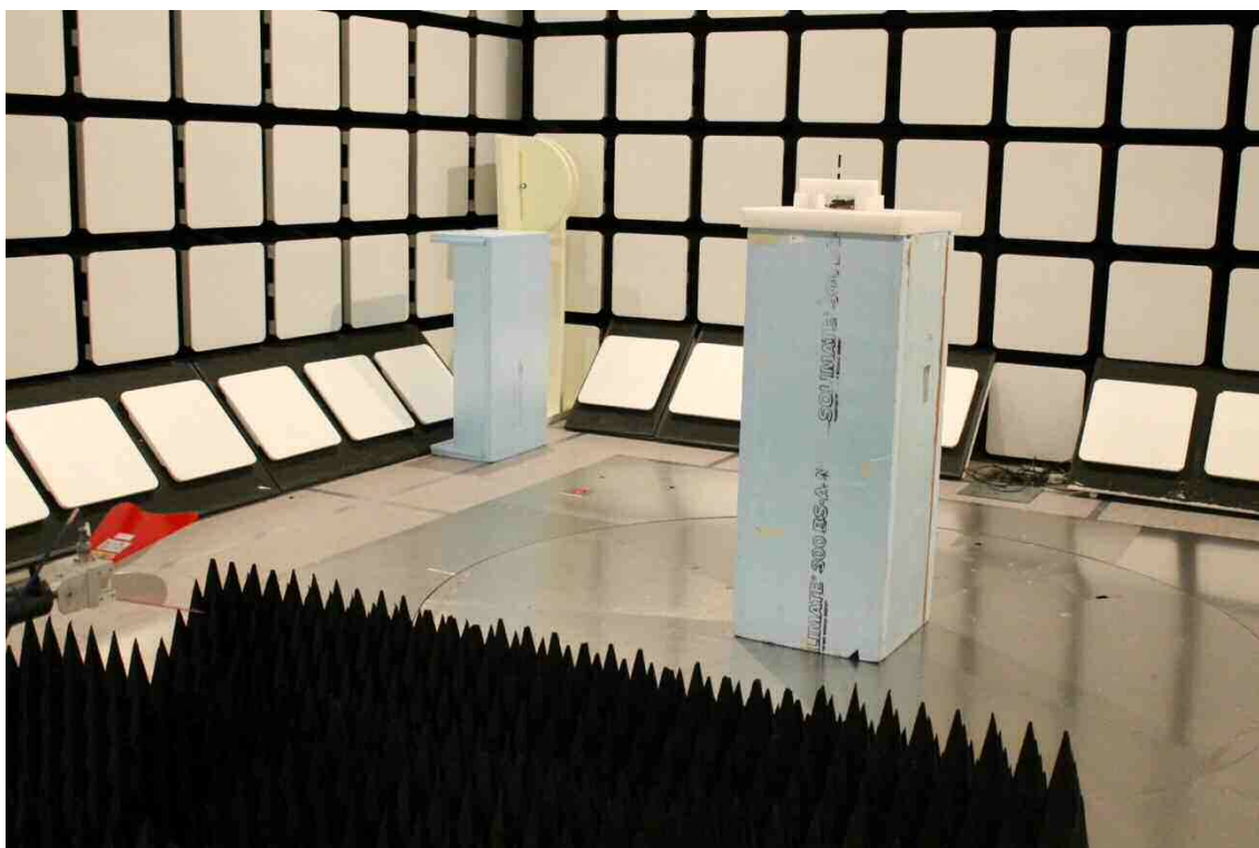
Photograph 2. Radiated Spurious Emissions 1 – 26.5 GHz (Antenna may vary)
