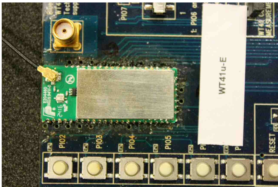
Photograph 7. The EUT
