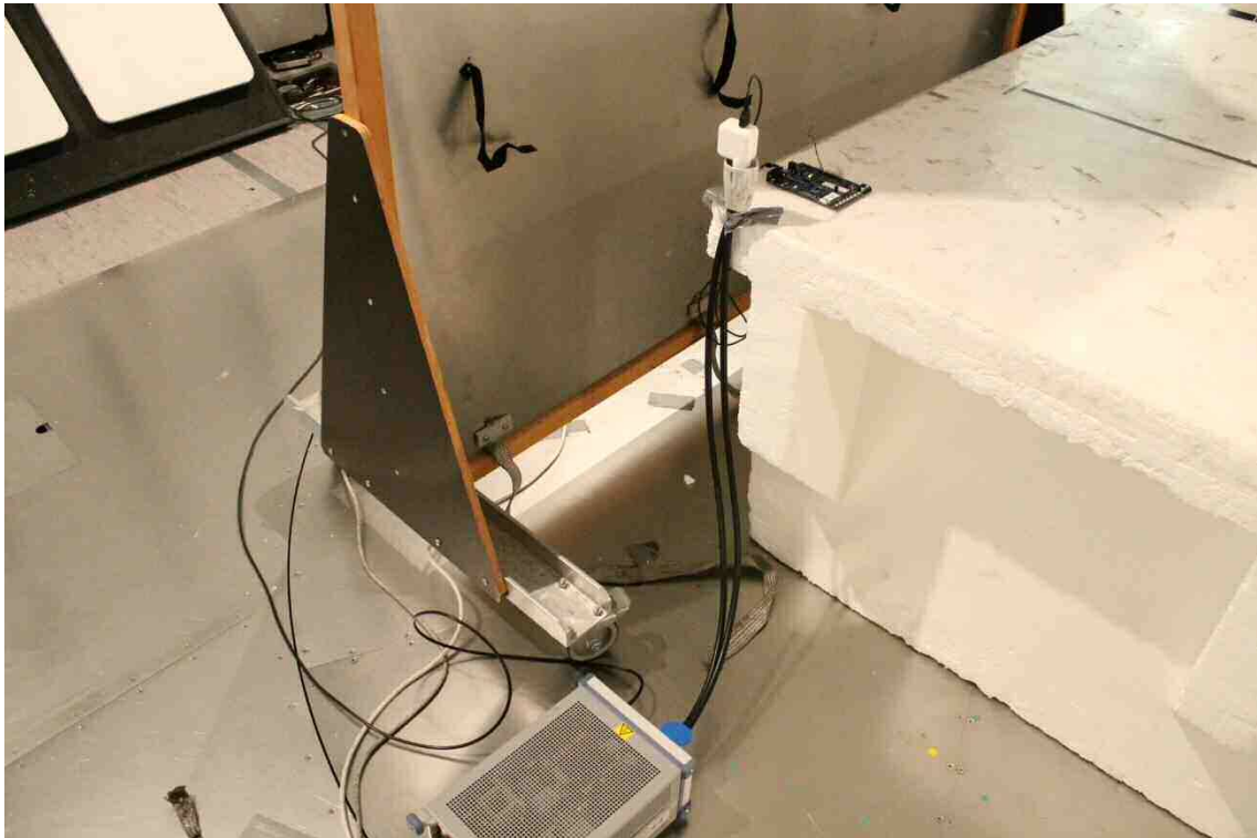
Photograph 5. Conducted emissions 150 kHz - 30MHz
