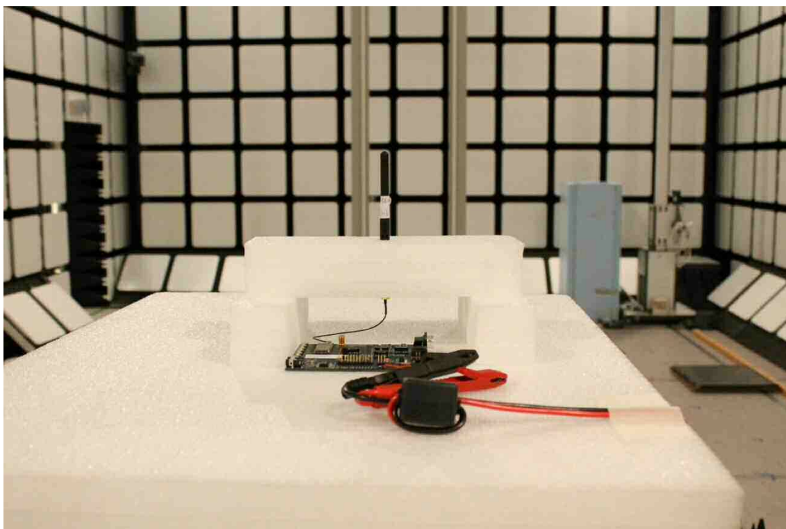
Photograph 4. EUT on table (WT11u-E)
