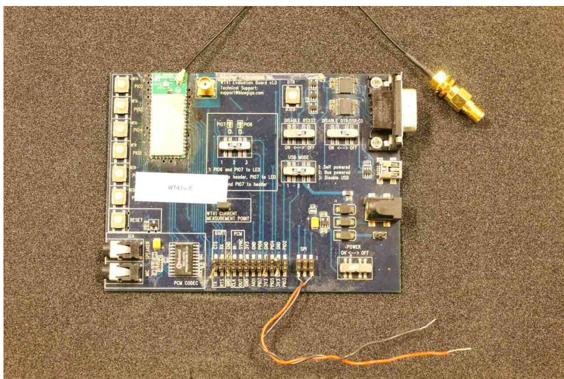
Photograph 8. The EUT placed on evaluation board
