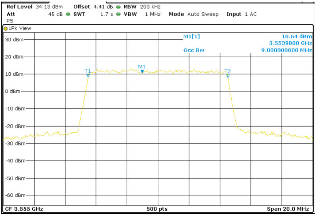
Band 42_BW10M_16QAM_Low Channel
