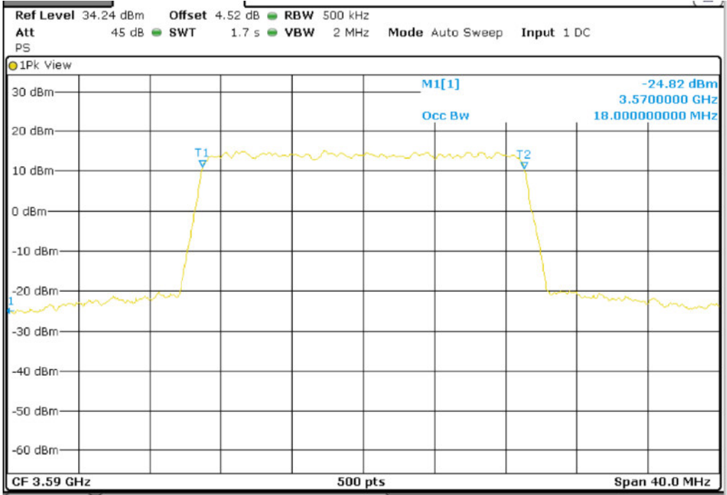
Band 42_BW20M_QPSK_High Channel
