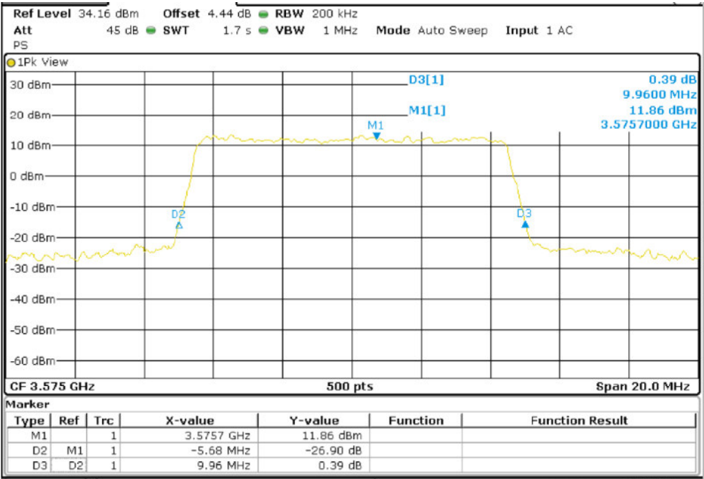
Band 42_BW10M_16QAM_Middle Channel
