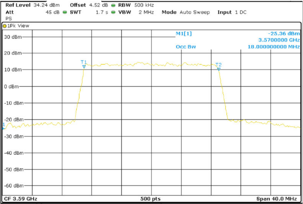
Band 42_BW20M_16QAM_High Channel
