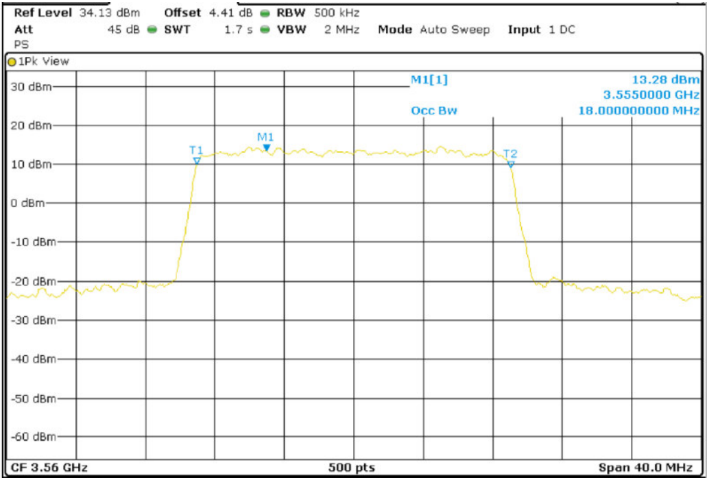
Band 42_BW20M_16QAM_Low Channel
