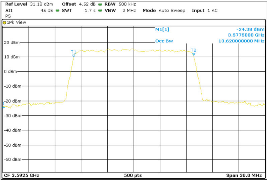
Band 42_BW15M_16QAM_High Channel
