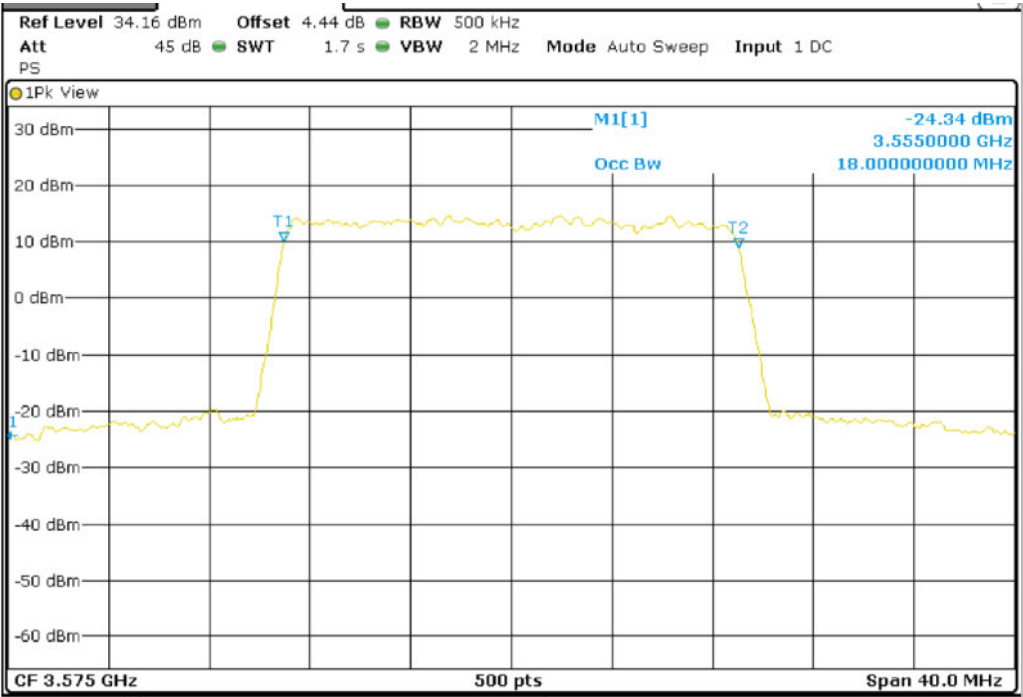
Band 42_BW20M_16QAM_Middle Channel
