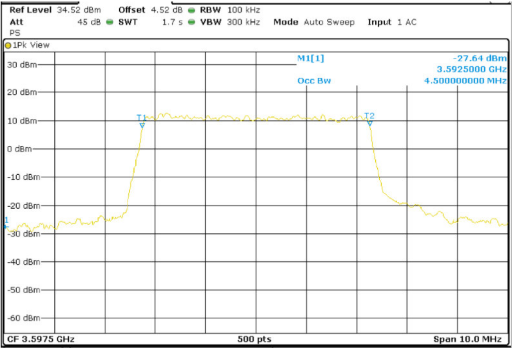
Band 42_BW5M_16QAM_High Channel
