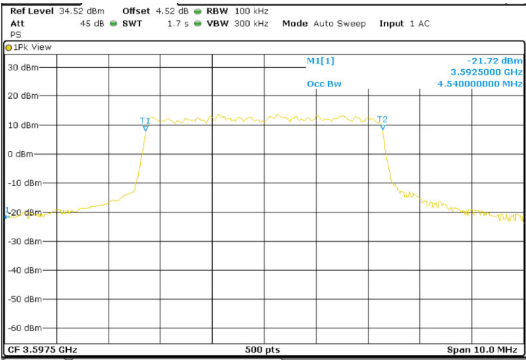
Band 42_BW5M_QPSK_High Channel
