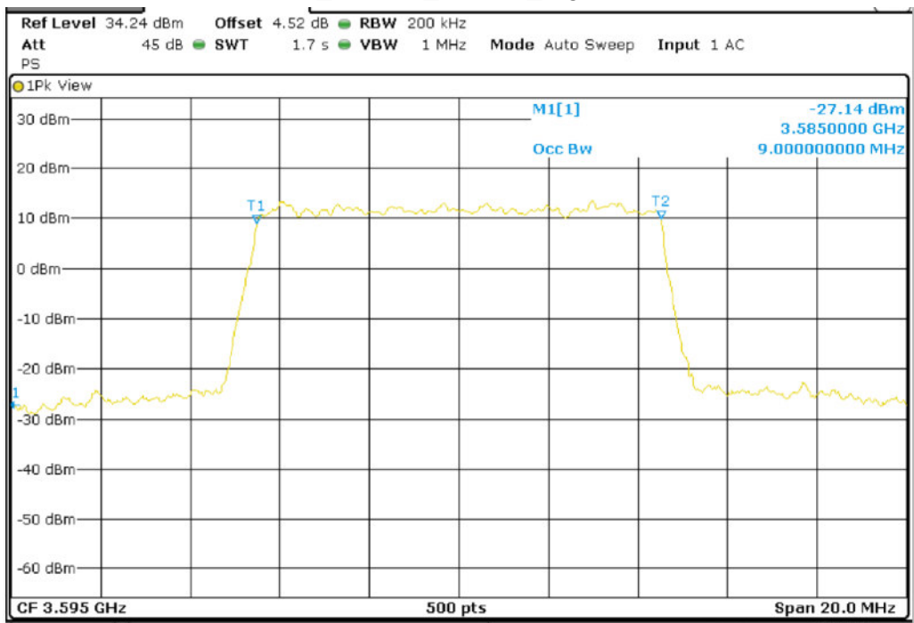
Band 42_BW10M_16QAM_High Channel
