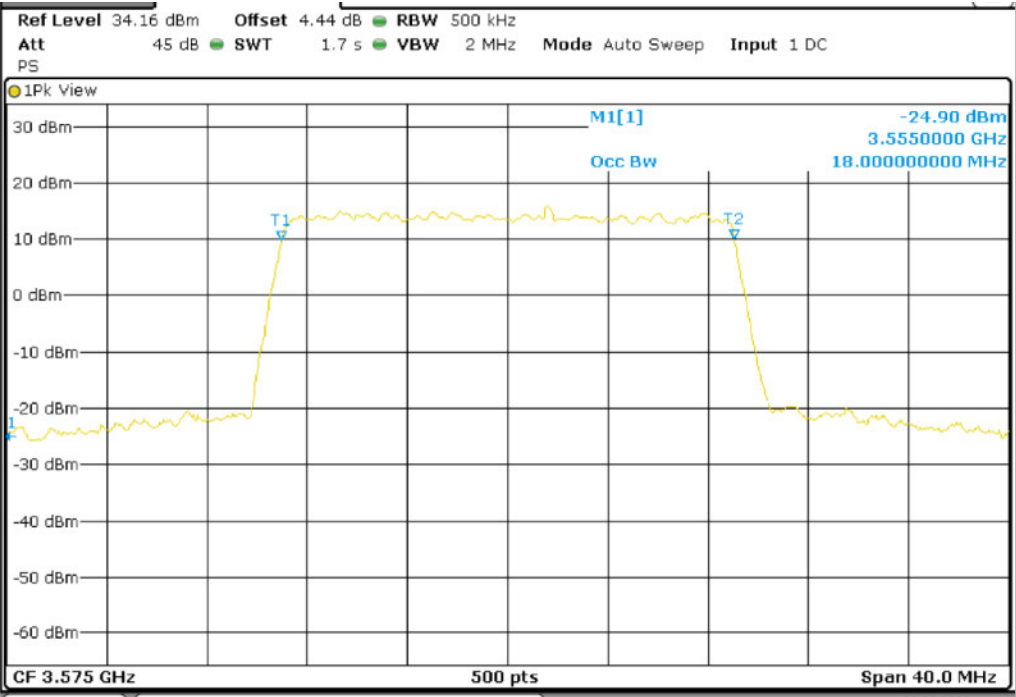
Band 42_BW20M_QPSK_Middle Channel
