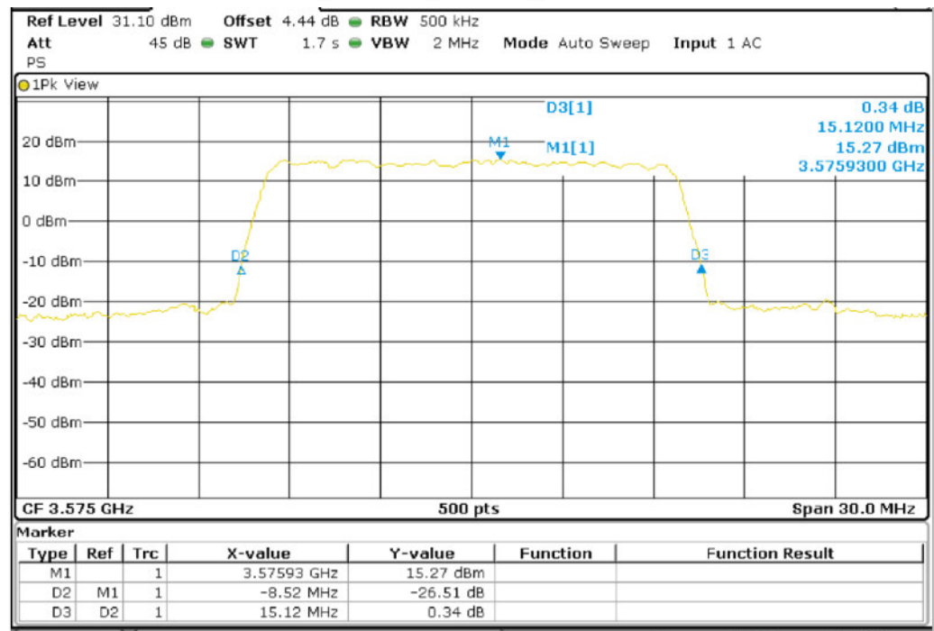
Band 42_BW15M_16QAM_Middle Channel
