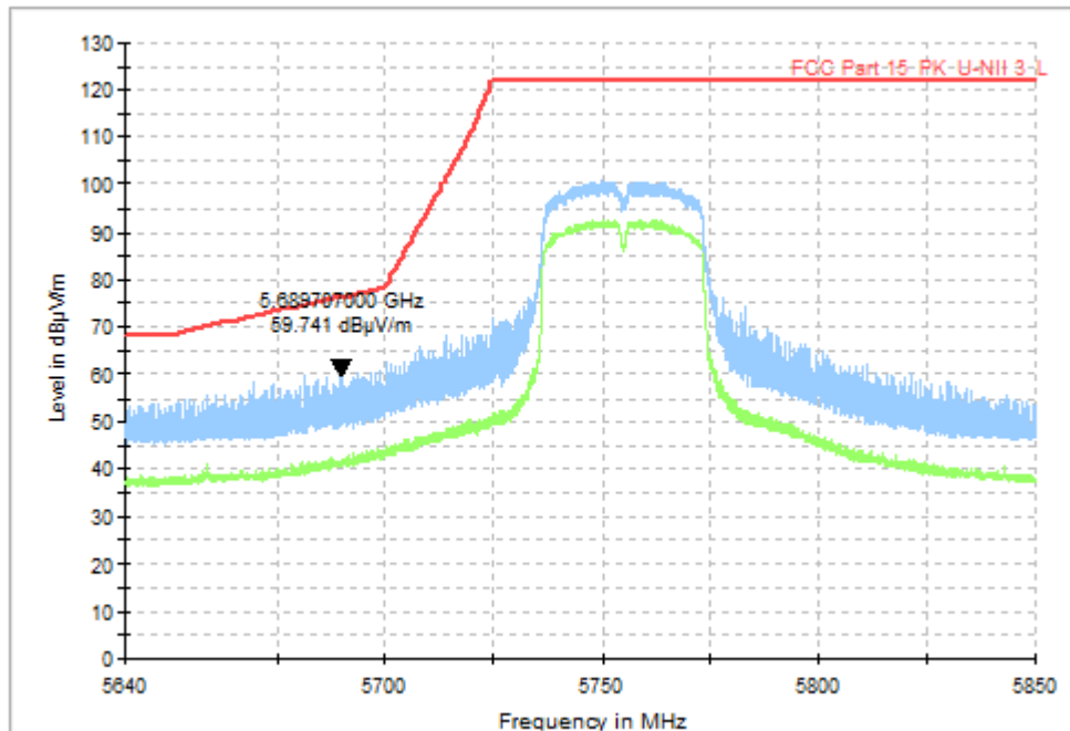
Fig. 59 Band Edges (802.11ac-VHT40, CH151 5755MHz)
