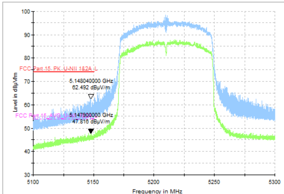
Fig. 61 Band Edges (802.11ac-VHT80, CH42 5210MHz)
