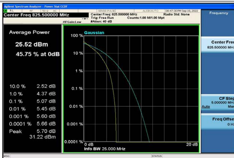
Band5-3MHz-QPSK-20415-15RB#0
