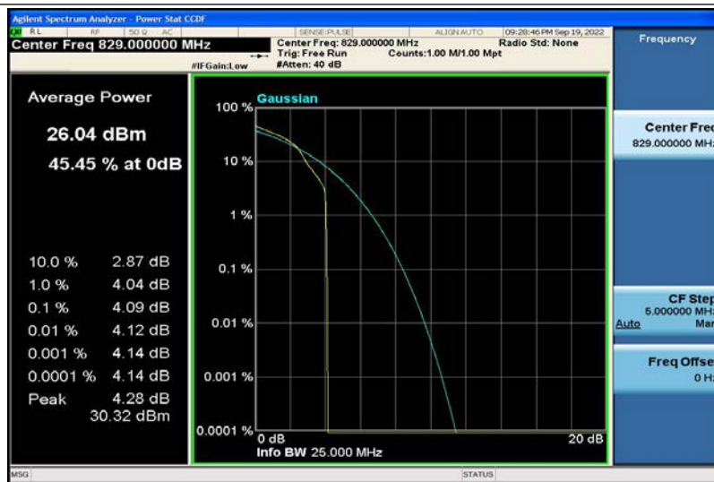
Band5-10MHz-16QAM-20450-1RB#0
