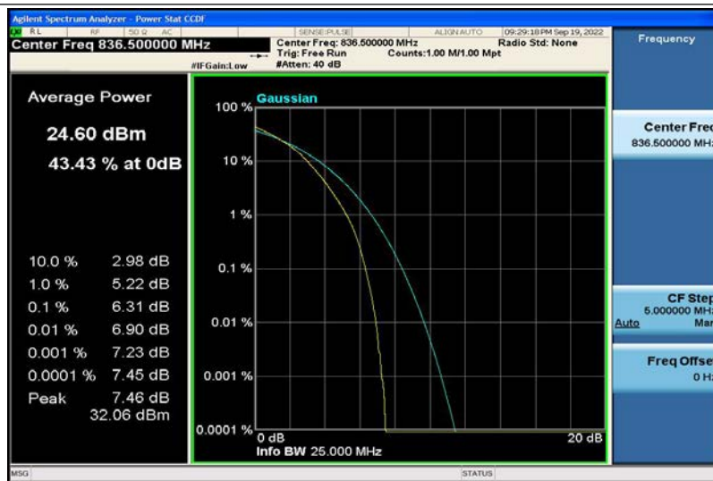
Band5-10MHz-16QAM-20525-50RB#0
