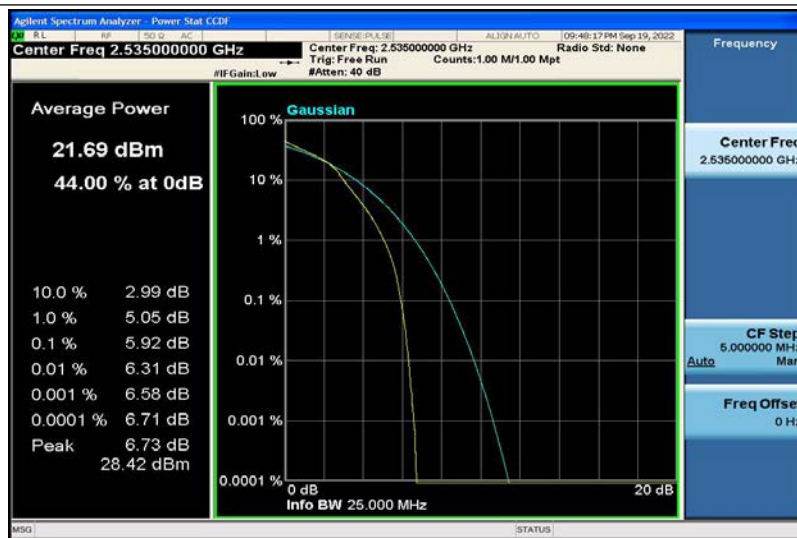
Band7-5MHz-16QAM-21100-25RB#0
