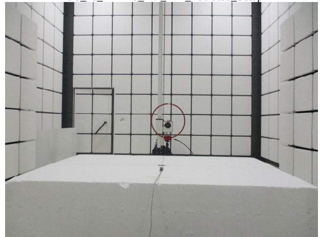
FCC_15_247+ IC_247_BLE_Radiated_Setup
