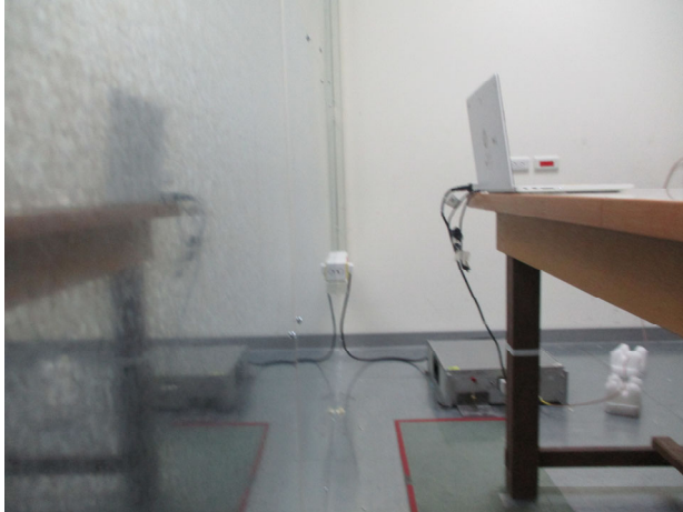
FCC_15_247+ IC_247_BLE_Radiated_Setup
