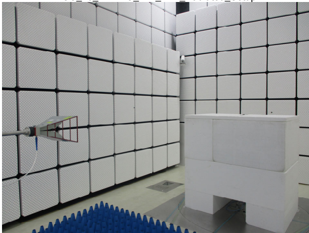
FCC_15_247+ IC_247_BLE_Radiated_Setup
