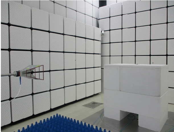
FCC_15_247+ IC_247_BT_Radiated_Setup
