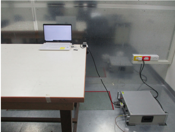
FCC_15_247+ IC_247_Conduction_Setup
