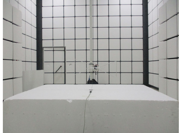
FCC_15_247+ IC_247_BLE_Radiated_Setup
