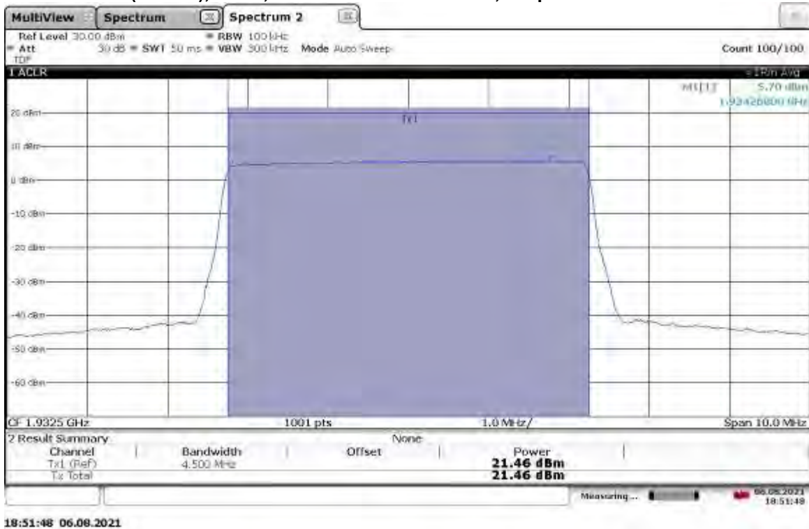
TM1.1-QPSK_5 MHz Bandwidth Slot 2 (Band 2), ANT1, Low Channel 1932.5 MHz, Output Power = 21.46 dBm
