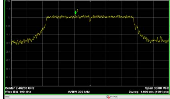
802.11g, Channel No.: 11
