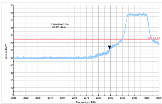
802.11g-Channel 1 Peak
