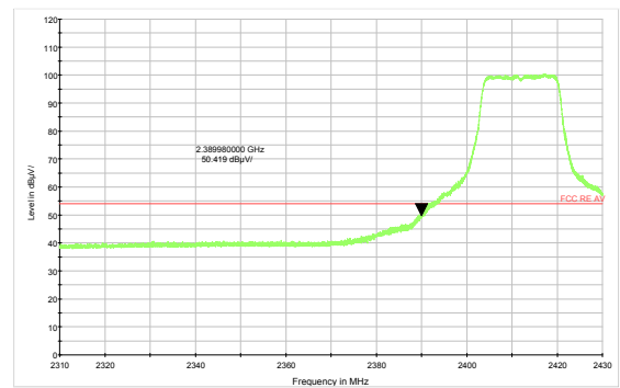
802.11g-Channel 1 Average
