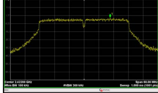
802.11n(HT40), Channel No.: 3
