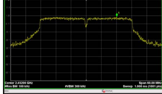
802.11n(HT40), Channel No.: 9
